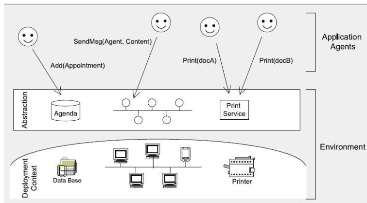
Fig. 2. Abstraction support level (from [?]).
