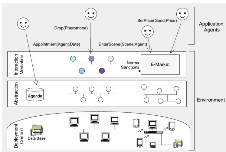
Fig. 3. Interaction-Mediation support level (from [?]).
