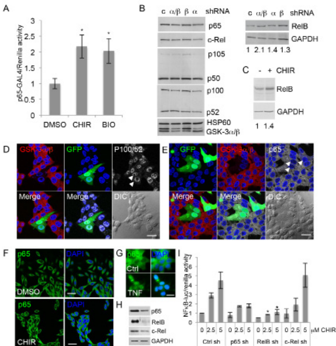
Figure 3: Inhibition of GSK-3 activates NFκB via RelB. (A) Gene reporter assays using extracts from 22Rv1 cells transfected with plasmids encoding p65-Gal4 Gal4-Luc, renilla and treated with vehicle (DMSO) or 5 μM CHIR99021 (CHIR) or 2.5 μM BIO-Acetoxime (BIO). Graph shows luciferase/renilla ratios normalized to DMSO; * p < 0.05 vs. DMSO; n = 2 . (B) Western blots of extracts from 22Rv1 cells transfected with control shRNA (c) or shRNAs targeting GSK-3 \alpha ( \alpha ), GSK-3 \beta ( \beta ) or both isoforms ( \alpha/\beta ), selected with puromycin for 72 h and probed for the indicated NFκB family proteins and HSP60 and GAPDH as loading controls. Numbers below the GAPDH blot indicate relative RelB signal normalized to GAPDH. Densitometry analysis (ImageJ) from 3 experiments indicated that silencing both GSK-3 isoforms together increased RelB 1.6 to 2.1-fold, compared to control shRNA ( p < 0.05 ). (C) Western blots of extracts from 22Rv1 cells treated with 2.5 μM CHIR99021 (CHIR) or vehicle (DMSO) for 16 h were probed for RelB and GAPDH as a loading control. Densitometry analysis from 3 experiments indicated that RelB was 1.4 to 2.3-fold higher in CHIR99021-treated cells than in DMSO-treated cells ( p < 0.05 ). (D, E) Immunostaining for GSK-3 \alpha and GSK-3 \beta (red) and p100/p52 (D) or p65 (E) (white) in 22Rv1 cells transfected with shRNAs to silence both GSK-3 isoforms and GFP plasmid (green) to visualize transfected cells. DAPI staining of nuclei is shown in blue. Arrows indicate cells silenced for GSK-3; scale bars 25 μm. (F) Immunostaining for p65 (green) in 22Rv1 cells treated with vehicle (DMSO) or CHIR99021 (CHIR) for 16 h. DAPI staining of nuclei is shown in blue; scale bar 25 μm. (G) Immunostaining for p65 (green) in 22Rv1 cells with vehicle (Ctrl) or TNF for 3 h. DAPI staining of nuclei is shown in blue; scale bar 62.5 μm. (H) Western blots of extracts from 22Rv1 cells transfected with control (left) or the indicated shRNA plasmid (right), selected with puromycin for 72 h and probed for p65, RelB and c-Rel; GAPDH was used as a loading control (blot shown is for RelB shRNA). (I) Gene reporter assays using extracts from 22Rv1 cells transfected with control (Ctrl), p65, RelB and c-Rel shRNAs, selected with puromycin for 72 h, then transfected with NFκB-luciferase and renilla and treated with DMSO or CHIR99021 at 2.5 μM and 5 μM. Graph shows luciferase/renilla ratios normalized to DMSO in Ctrl cells; * p < 0.05 vs. Ctrl sh at the same dose of CHIR99021; n = 2 .
