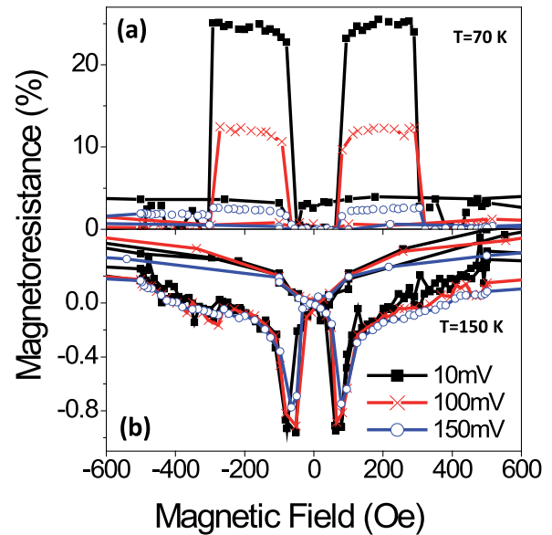
FIG. 7. (Color online) Dependence of magnetoresistance on the applied bias voltage for an annealed junction of 9 \times 18 \mu\text{m}^2 and MgO thickness of 2.4 nm. (a) At 70 K, the positive TMR notably decreases with increasing voltage bias. (b) At 150 K, the negative contribution is rather insensitive to changes of the voltage bias.
