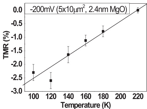
FIG. 5. Temperature dependence of the negative TMR (measured at -200 \text{ mV} for the same junction as in Fig. 4). The line is a guide to the eyes.
