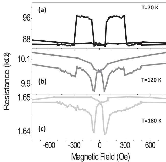
FIG. 6. Dependence of magnetoresistance on the applied magnetic field at a fixed applied voltage bias of 100 mV and different temperatures for an annealed junction of 9 \times 18 \mu\text{m}^2 and MgO thickness of 2.4 nm. (a) At 70 K, a positive TMR with well-defined antiparallel magnetizations of both LSMO and Fe electrodes is observed. (b) At 120 K, the TMR is mainly negative but a visible positive contribution persists. (c) At higher temperatures, only the negative magnetoresistance remains.
