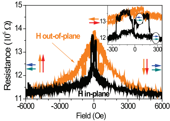
FIG. 8. (Color online) Dependence of the magnetoresistance on the direction of the applied magnetic field for a fixed applied voltage bias of -50 mV at T = 10 K [ 5 \times 15 \mu\text{m}^2 junction from an Fe (20 nm)/MgO(1.2 nm)/(42) LSMO stack]. The magnetic field was applied parallel to the surface, along the [100] Fe easy axis ( H in-plane) and perpendicular to the film ( H out-of-plane). Inset shows zoom for lower magnetic fields, for clarity.
