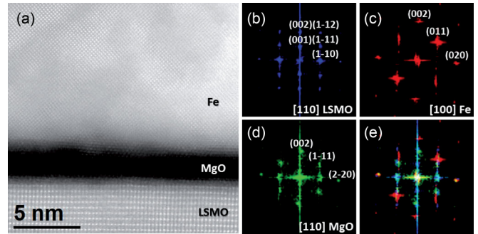
FIG. 1. (Color online) (a) HAADF-STEM image of a cross section of a postannealed \text{La}_{0.7}\text{Sr}_{0.3}\text{MnO}_3/\text{MgO}/\text{Fe} heterostructure evidencing the crystallinity of the different layers. However, the MgO/Fe interface is blurred and rough evidencing some structural disorder. (right) Power spectra obtained on the different layers forming the heterostructure: (b, blue) LSMO, (c, red) Fe, and (d, green) MgO. (e) The RGB power spectra contains the previous spectra overlapped showing their epitaxial relationship.
