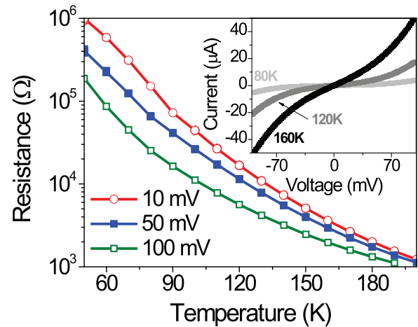
FIG. 3. (Color online) Temperature dependence of the resistance of the LSMO/MgO/Fe annealed junctions in the low- T regime for different voltage bias values. Inset shows nonlinear I - V curves obtained for different temperatures (80, 120, and 160 K).
