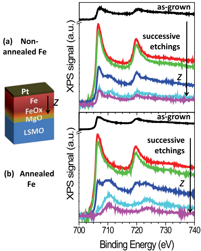
FIG. 2. (Color online) XPS spectra in the Fe 2p region of a Pt/Fe/MgO/La 0.7 Sr 0.3 MnO 3 /STO stack for different sample preparation conditions: (a) Fe grown with no in situ annealing after deposition and (b) Fe grown with an in situ annealing at 400 °C for 30 min after the deposition.
