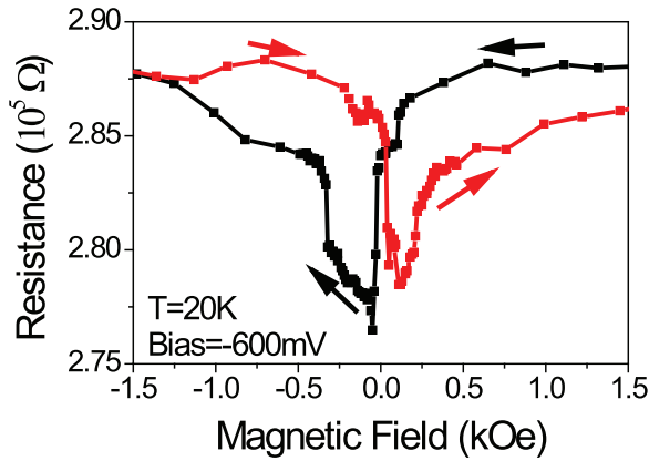
FIG. 4. (Color online) TMR response of a 5 \times 10 \mu\text{m}^2 -sized Fe/MgO(2.4 nm)/LSMO nonannealed magnetic tunnel junction.
