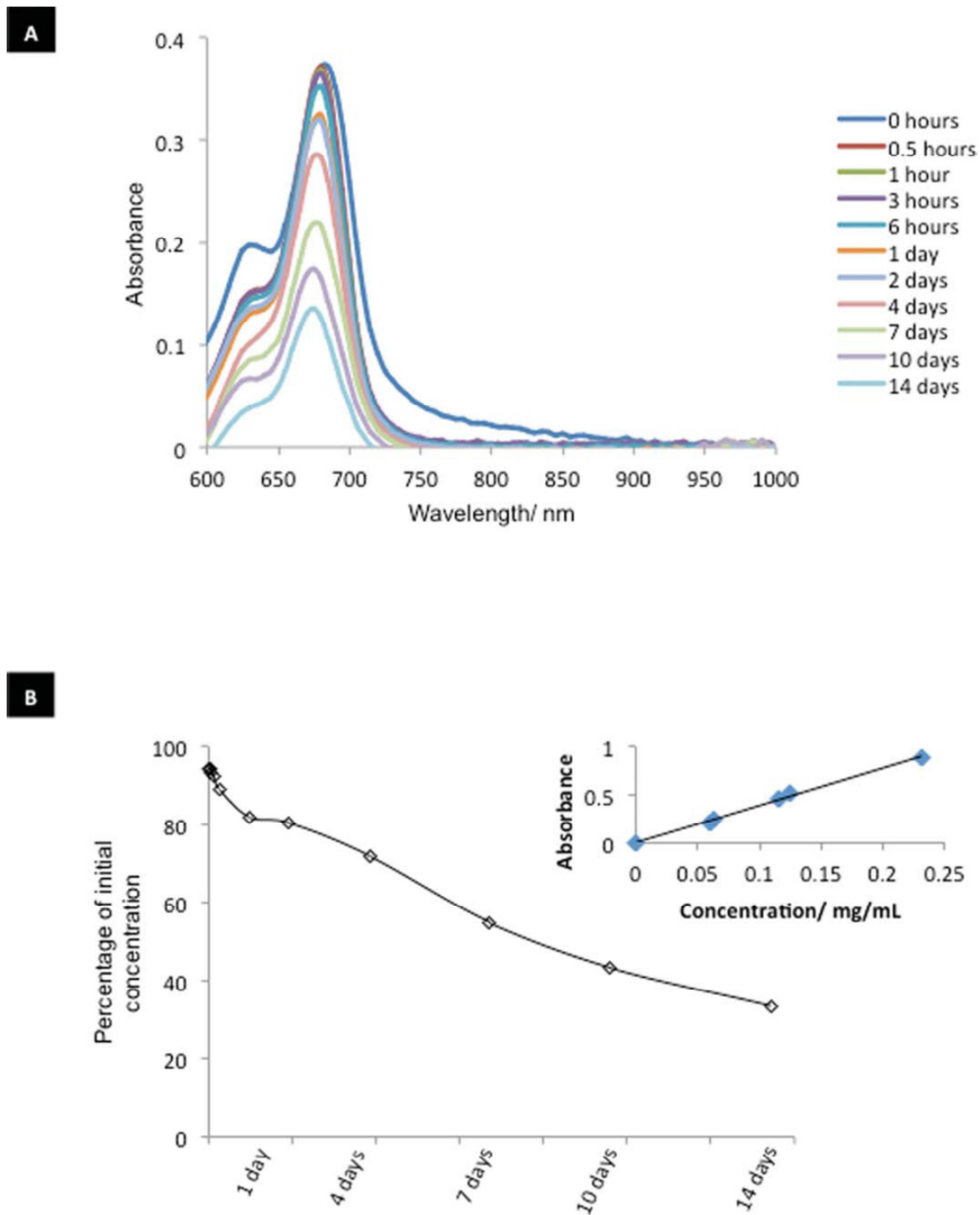
Fig. 2 UV-vis spectroscopy of KRK PNFs. Labelled KRK PNFs were incubated in rat plasma–PBS (1 : 1) and measured by UV absorbance. The percentage of intact fiber was measured by means of a calibration curve (inset).
