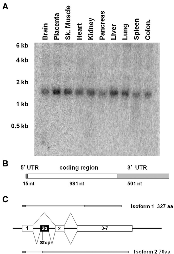
Fig. 2. Characterization of RNA steady-state levels, transcript isoforms, and gene structure of human COQ5 . (A) Northern blot analysis of COQ5 expression in different tissues. Each lane contains 200 ng of polyA + mRNA. (B) Schematic structure of the principal transcript of human COQ5 as determined by RACE experiments. (C) Genomic structure of the 5' region of COQ5 showing the alternatively spliced exon 2b and the resulting proteins.
