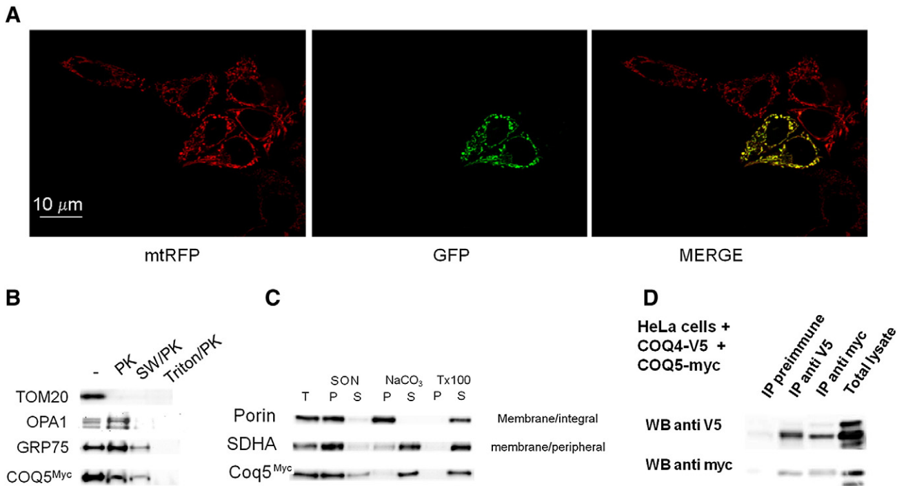
Fig. 3. Human COQ5 is located within the mitochondrial matrix and is peripherally associated with the inner membrane. (A) Co-localization of COQ5-GFP fusion proteins transiently expressed from pCOQ5-GFP in HeLa cells stably expressing mitochondria targeted RFP (mtRFP). (B) Proteinase K (PK) protection assays. Mitochondria were subjected to PK treatment directly after isolation and only outer membrane proteins are degraded (e.g. TOM20). Alternatively, mitochondria were treated with PK after treatment with hypotonic solution, which causes swelling (SW), and renders proteins of the inter-membrane space (e.g. OPA1) accessible to PK; or after treatment with a detergent (Triton X-100) which disrupts all mitochondrial membranes and allows PK degradation of all compartments including matrix proteins (e.g. GRP75). The susceptibility of COQ5 to PK follows the same pattern as GRP75, a mitochondrial matrix protein. (C) Membrane association assays. Mitochondrial membranes were prepared by sonication followed by centrifugation (12,000 g for 10 min) to generate pellet and supernatant fractions: isotonic buffer conditions (SON), NaCO 3 treatment (which solubilizes peripheral membrane proteins), or Triton X-100 (which solubilizes integral membrane proteins). Aliquots of the supernatants (S) and pellets (P) were separated by SDS-PAGE and proteins were detected with the designated antibodies. A sample of the total membrane preparation (T) was included as control. (D) Mitochondrial extracts of HEK293 cells co-expressing COQ5-myc and COQ4-V5 were immune-precipitated with anti-myc, anti-V5 or with pre-immune sera. Immune-precipitates were separated by SDS-PAGE, transferred to membranes and the tagged-polypeptides were detected with either anti-V5 or anti-myc antibodies.
