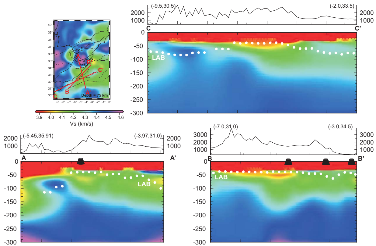
Figure 9. Cross sections through the Atlas Mountains indicated on the Vs map at 75 km depth. The crustal velocities less than 3.9 km/s are set to a constant 3.9 km/s for display. Horizontal segments represent the tectonic zones (ER: External Rif; MM: Moroccan Meseta; MA: Middle Atlas; HA: High Atlas). Black cones represent the position of Cenozoic volcanics. White dots indicate the depth of the estimated LAB (see text and Figure 10).
