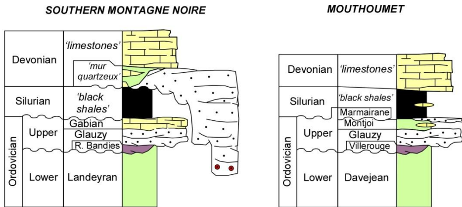
Figure 5. Schematic stratigraphic logs of the Lower Ordovician–Devonian in the southern Montagne Noire and Mouthomet massif.
