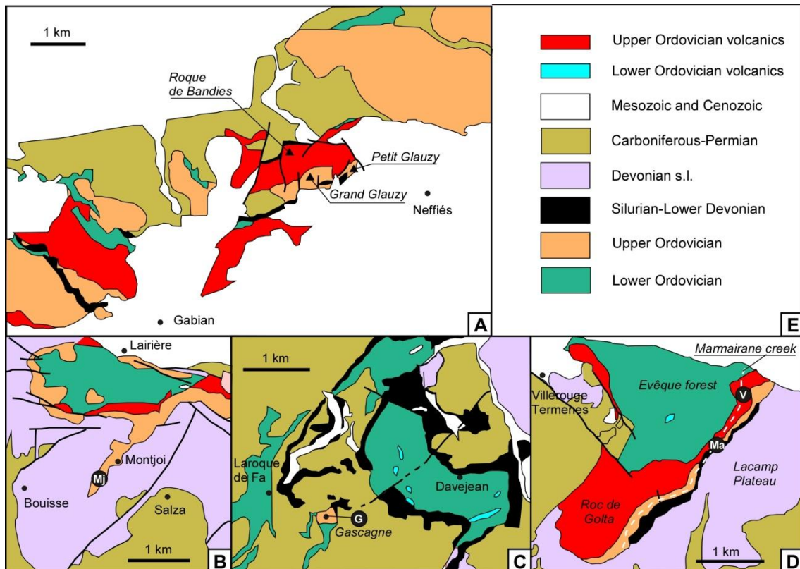
Figure 3. Geological sketches of the Cabrières klippe in the southern Montagne Noire and Mouthoumet study areas. A. Pre-Variscan outcrops in the vicinity of Neffiés, Cabrières klippe. B. Surroundings of Montjoi, Mouthoumet parautochthon. C. Davejean and Laroque de Fa, Félines-Palairac slice. D. Villeroque-Termenès, Félines-Palairac slice. E. Legend; modified from Berger (1982), Bessière et al. (1984, 1989), Bessière and Baudelot (1988) and Berger et al. (1990, 1993, 1997). Abbreviations- G: Gascagne stratotype, Ma: Marmairane stratotype, Mj: Montjoi stratotype, V: Villeroque stratotype. See Figure 1 for setting of mapped areas.
