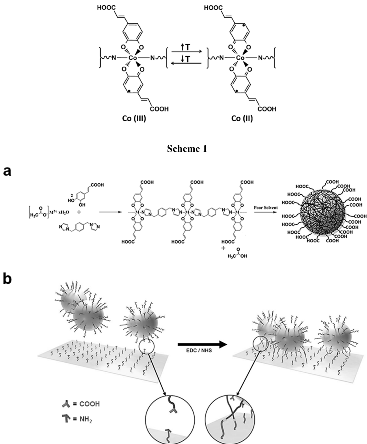
Figure 1. a) Schematic of the formation of polymeric chains for CPP-Co and structuration into a nanostructure by fast precipitation. b) Schematic of the attachment of carboxyl functionalized nanoparticles onto a gold surface previously covered with a monolayer of amino- terminated alkyl chains through carbodiimine mediated coupling reaction.
