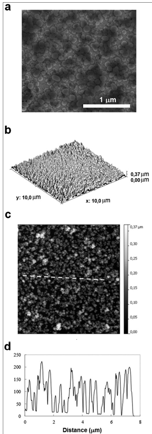
Figure 2. a) SEM image of the CPP-Co chemically attached to the surface after condensation reaction; b-c), 3-D AFM topography image and topography image of the surface densely covered with CPP-Co , respectively; d) Height profile corresponding to white dashed line in (c).
