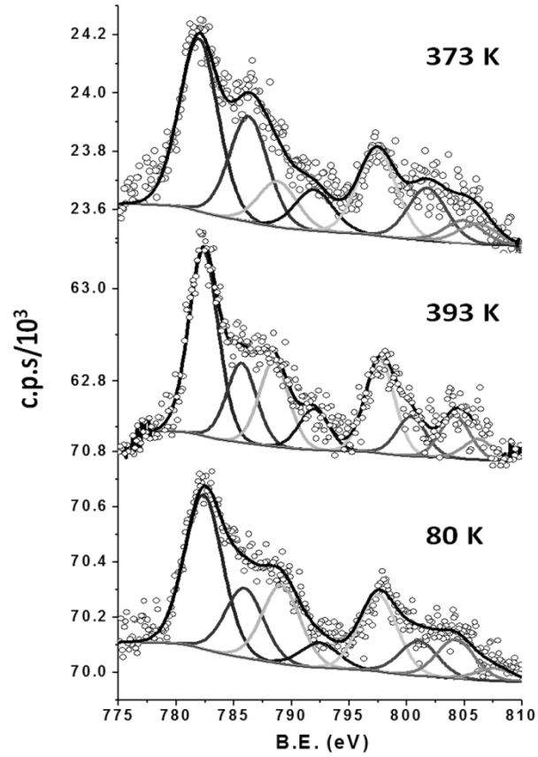
Figure 3. Variable-temperature Co 2p XPS spectra of CPP-Co nanoparticles attached to a gold surface along with best-fit components.
