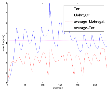
Fig. 7 Flows from the two rivers after using temporal coordination with x-time and y-flow axis
