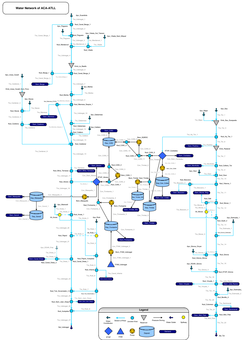
Fig. 1 Aggregate diagram of Catalunya Regional Water Network
