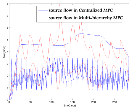
Fig. 8 Source flows comparison between Multi-hierarchical MPC and Centralized MPC
