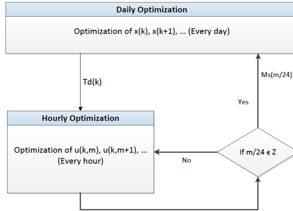
Fig. 4 Upper and Lower layer optimizations of multi-layer MPC
