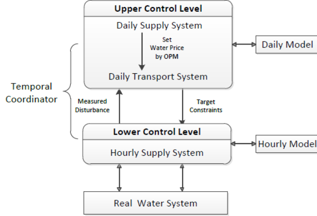
Fig. 2 Temporal hierarchical coordinating structure
