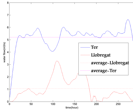
Fig. 6 Flows from the two rivers before using temporal coordination with x-time and y-flow axis
