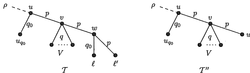
Fig. 5. The structure of \mathcal{T} and \mathcal{T}'' in Case 2. The labelling of \mathcal{T}'' is induced by \mathcal{T} , except for w which is unlabelled in \mathcal{T} , and labelled \phi^{-1}(\ell') in \mathcal{T}'' .
