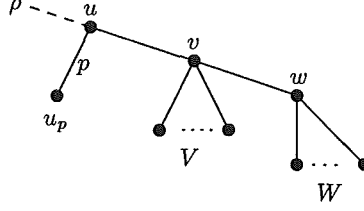
Fig. 4. The vertices surrounding the edge (v, w) .
