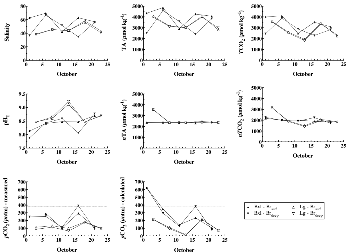
Figure 5. Evolution of salinity, \text{pH}_T , TA (in \mu\text{mol kg}^{-1} ), n\text{TA} (TA normalized to a salinity of 34, in \mu\text{mol kg}^{-1} ), calculated T\text{CO}_2 (in \mu\text{mol kg}^{-1} ) and nT\text{CO}_2 ( T\text{CO}_2 normalized to a salinity of 34, in \mu\text{mol kg}^{-1} ), and measured and calculated p\text{CO}_2 (in \mu\text{atm} ) in surface and deep brine sackholes from the Brussels (Bxl) and Liège (Lg) sites. The dotted line represents the atmospheric p\text{CO}_2 in October 2007.
