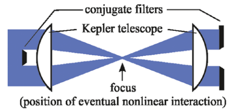
Figure 1. Schematic of the nonlinear filter.
