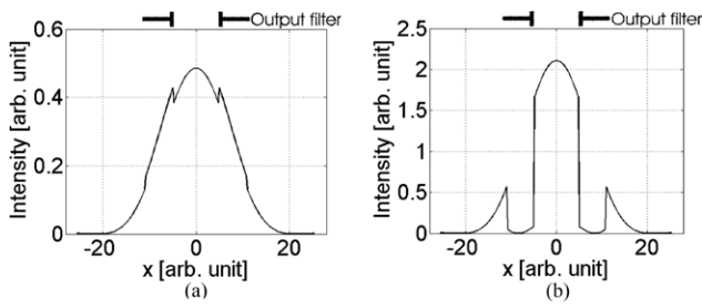
Figure 3. Output of the confocal telescope when the relative amplitude (a) and the phase (b) of the central lobe of the diffraction pattern are modulated (for details see text).
