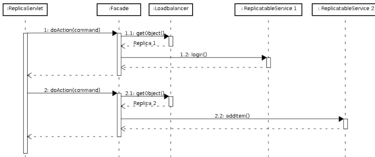
Fig. 6 Communication among Load Balancer, HTTP Wrapper and Replicas
