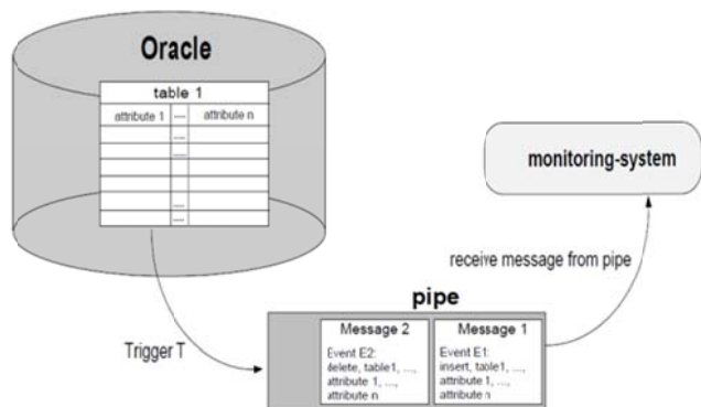
Fig. 3 Monitoring: Triggers and Callbacks
