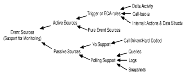
Fig. 2 Classification: Monitoring Support
