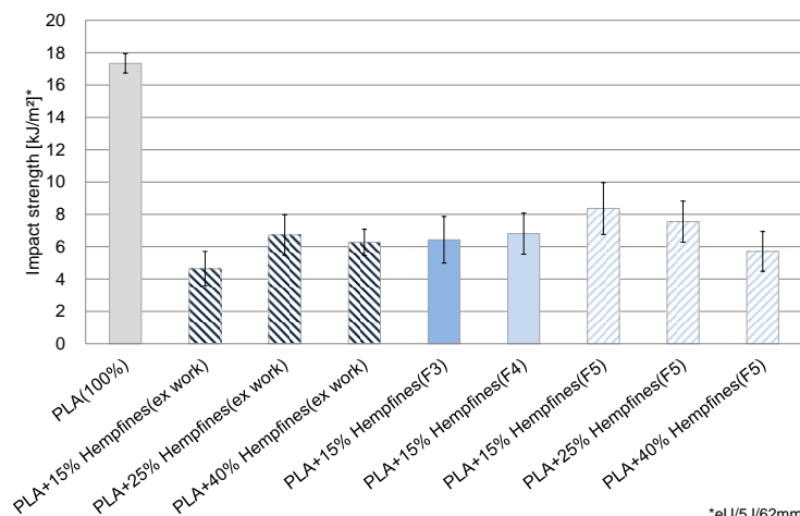
Figure 3. Impact strength in [kJ/m 2 ]
