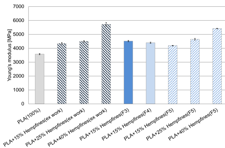
Figure 2. Young's modulus in MPa
