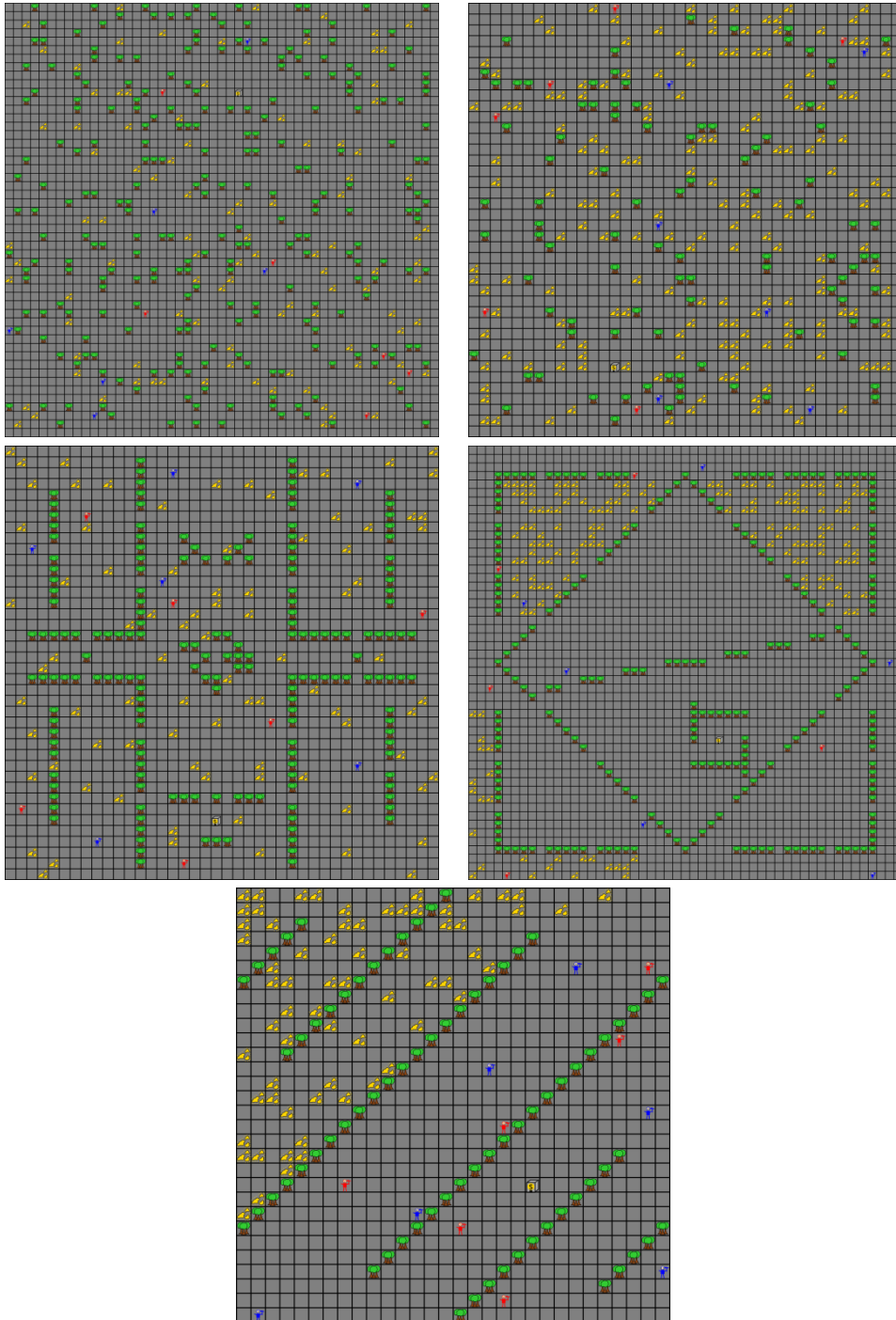
Figure 1: Initial simulation scenarios Park , Meadow , Semiramis , Fence and Overkill (left → right, up → down)
