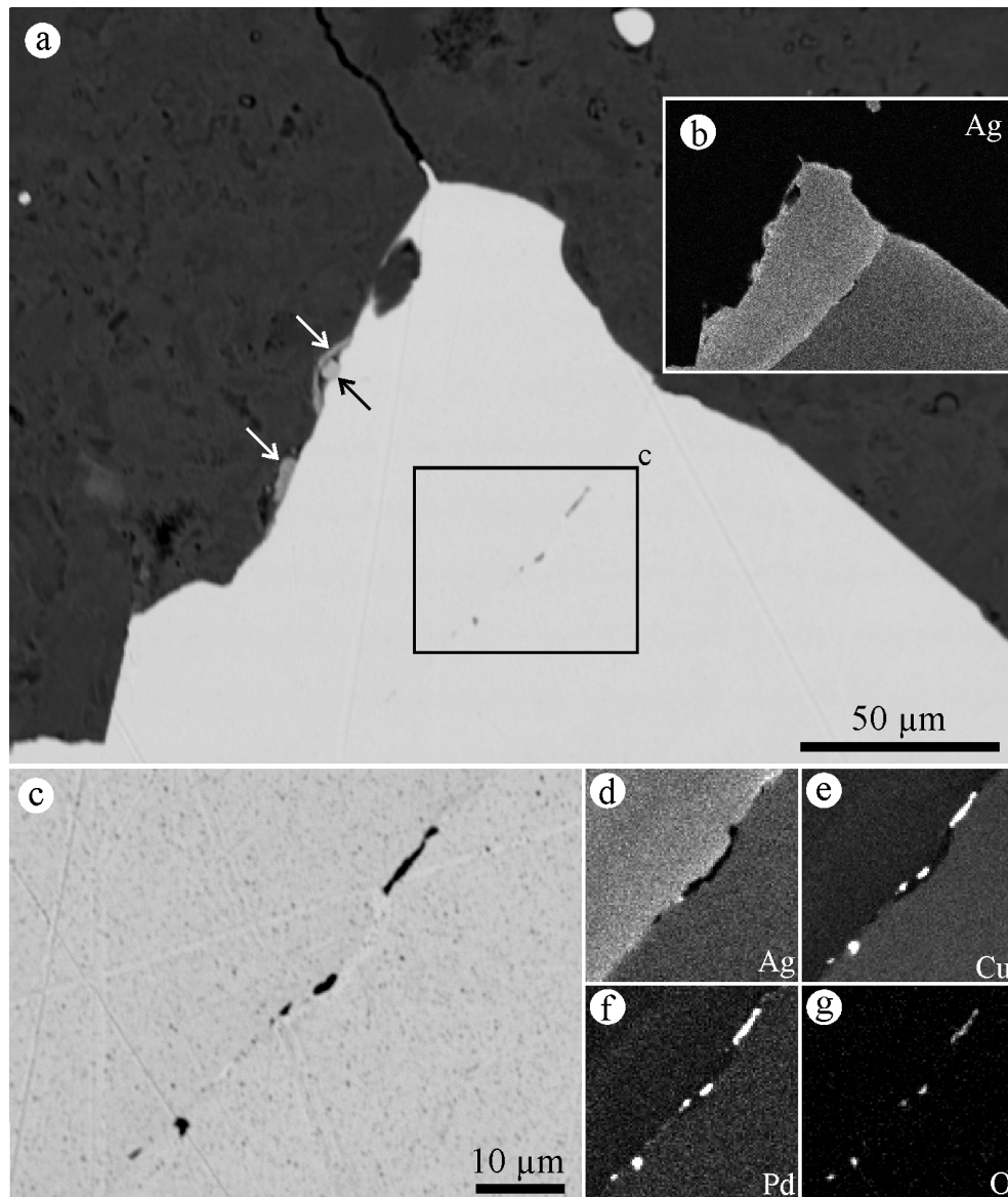
Fig. 15: (a) BSE image of the area squared in Figure 12d at the contact between gold (white) and an envelope of barium-bearing manganese oxide (dark grey). Note that gold protrudes into the Mn–Ba–O phase. Masses of Pd–O phase (white arrows) occur on the surface of gold, as isolated patch and as coating on an As-bearing Pd–Sb phase (black arrow). (b) X-ray element distribution of AgL \alpha . (c) BSE image of the area squared in (a), with X-ray element distributions of (d) AgL \alpha , (e) CuK \alpha , (f) PdL \alpha and (g) OK \alpha .
