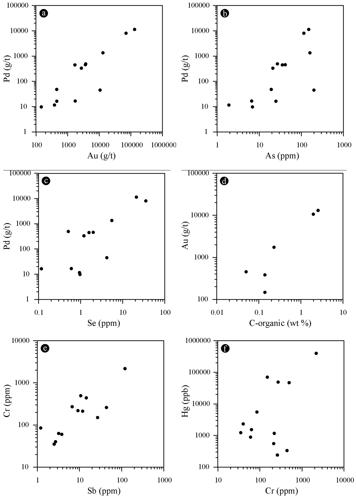
Fig. 52: Variation diagrams for some elements from ore samples of drill core SP-32. Data are from Tables 18 and 19 and CABRAL et al. (2002a).
