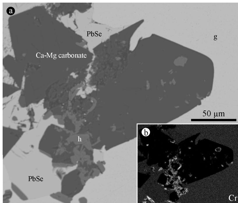
Fig. 22: (a) BSE image of a brecciated aggregate of clausenthalite, PbSe, Ca-Mg carbonate and chromiferous hematite, h. (b) X-ray mapping for CrK \alpha (sample Au-11).
