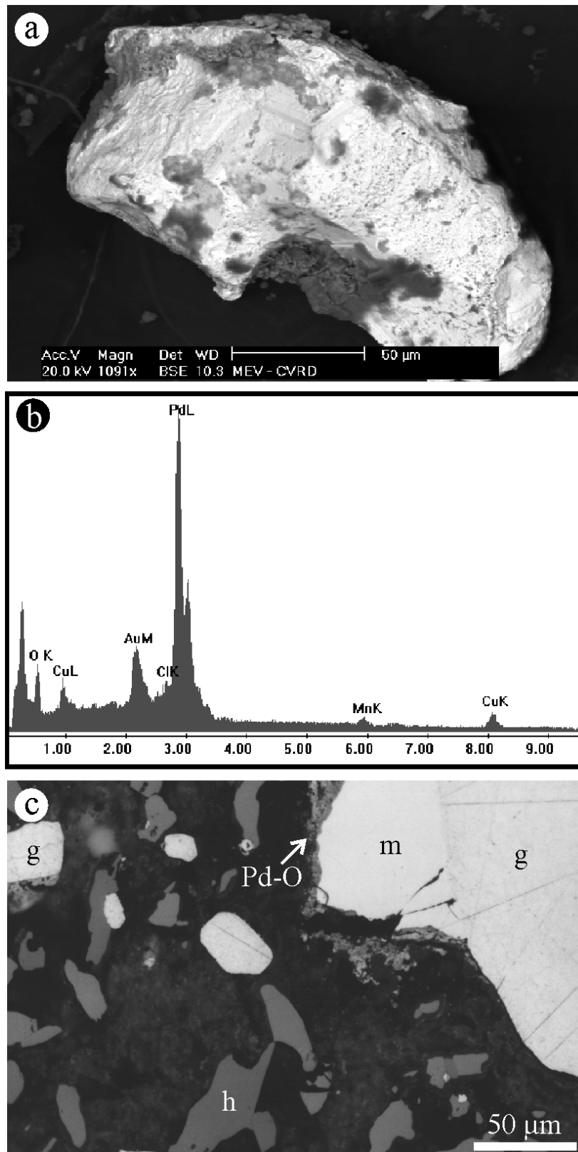
Fig. 23: (a) BSE image of a grain of ouro preto (black gold), characterised by coating of Pd-O material (grey, top) and iron oxyhydroxide (dark grey, bottom). (b) ED spectrum of the Pd-O coating shown in (a). (c) Gold, g, and specularite, h, within goethite-like groundmass (shades of grey), reflected light, oil immersion. Mertieite-II, m, is rimmed by a greyish halo of Pd-O. The Pd-O halos on crystals of Pd-Sb-As, together with iron oxides, give the dark colour to the ouro preto of Gongo Soco.
