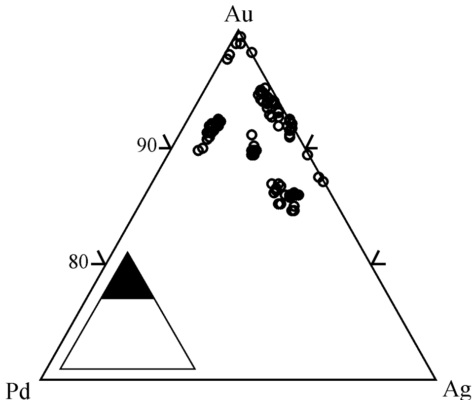
Fig. 13: Composition of nuggets and aggregates of gold from Tables 2 and 3 (in wt %).
