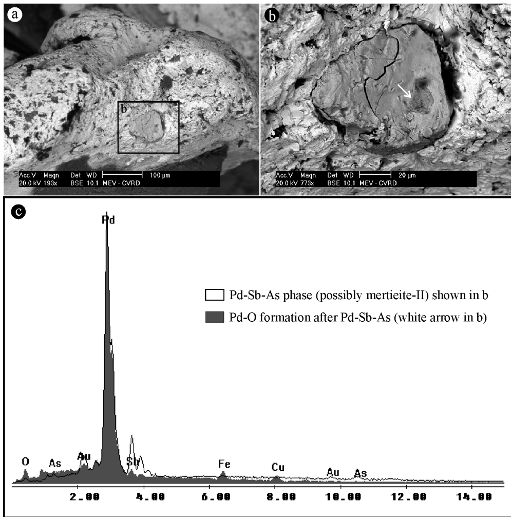
Fig. 19: (a) BSE image of a gold nugget, sample Au-6. (b) BSE image of the area squared in (a) to highlight that the Pd-Sb-As mineral is microfractured and has a Pd-O coating (white arrow). (c) Energy dispersive (ED) spectra of the Pd-Sb-As mineral and its Pd-O coating.
