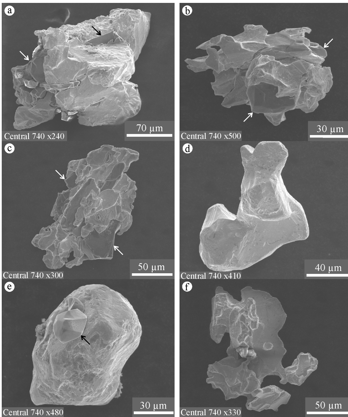
Fig. 32: Secondary electron (SE) images of gold from Central, level 740. (a), (b), (c) Gold intergrowth with specularite (arrows). (d) Dendritic crystal of gold. (e) Euhedral crystal of gold (arrow) on the surface of anhedral gold. (f) Gold with irregular protuberances.
