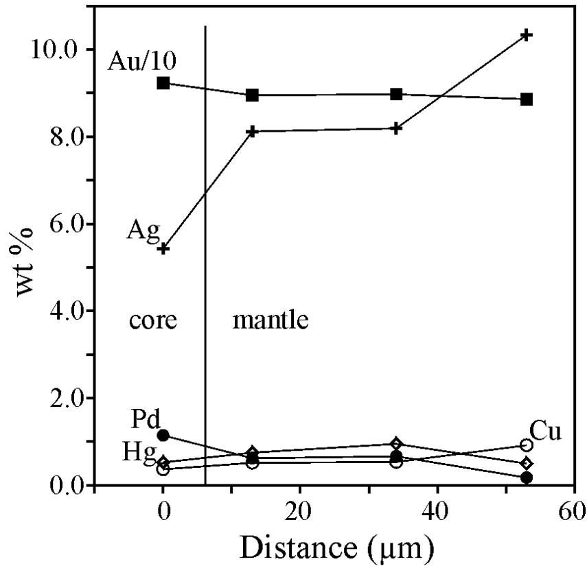
Fig. 16: Composition of gold across the contact between the core and mantle shown in Figure 15 (microanalyses 3, 4, 5 and 6 of Table 2).
