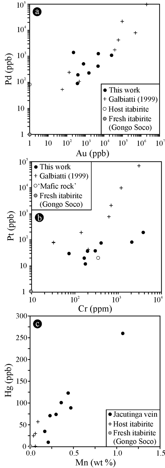
Fig. 41: Variation diagrams. (a) Au vs. Pd, (b) Pt vs. Cr and (c) Hg vs. Mn for jacutinga veins (data from Table 15 and GALBIATTI 1999), host itabirite (Table 15) and reference fresh itabirite (Gongo Soco, Table 10). In (b) the 'mafic rock' (crumbly, ochreous schist, Table 15) is plotted for comparison.
