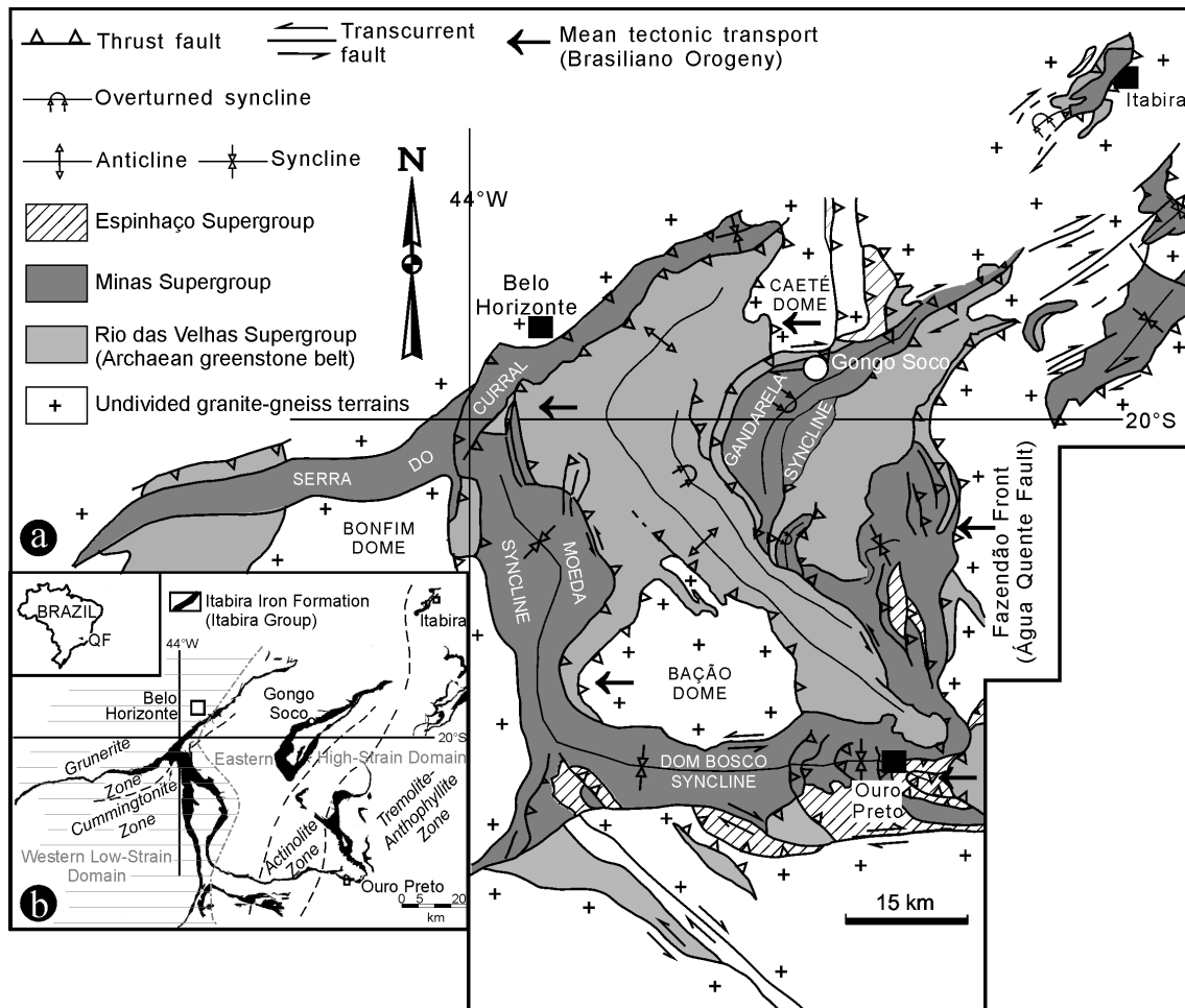
Fig. 6: (a) Simplified geological map of the Quadrilátero Ferrífero (after ROSIÈRE et al. 2001). (b) Distribution of the Itabira Iron Formation (Itabira Group), with metamorphic zones (dashed lines, after PIRES 1995) and strain domains (after ROSIÈRE et al. 2001).
