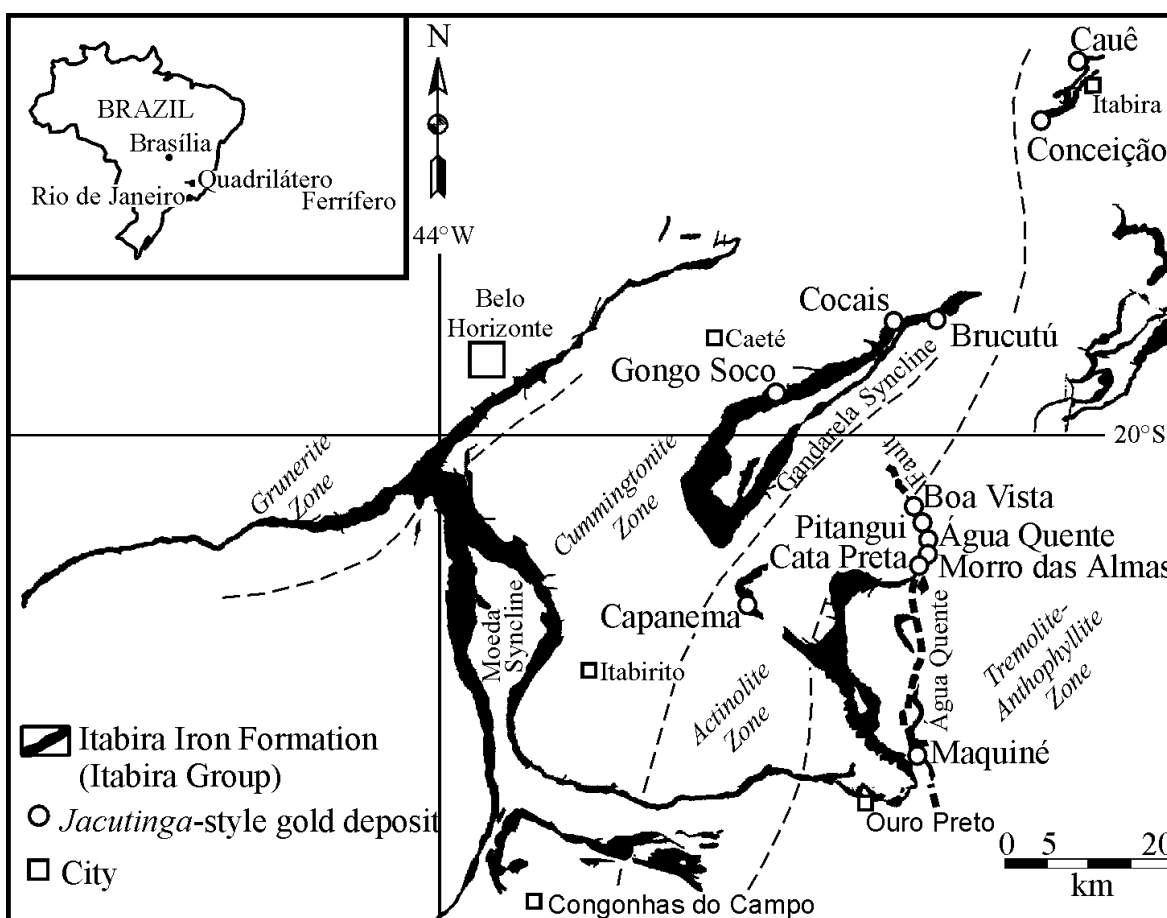
Fig. 1: Location of jacutinga -style gold deposits (open circles) in relation to the Itabira Iron Formation (Itabira Group), shown in black (after DORR 1969), with the metamorphic zones of PIRES (1995), dashed lines. Gold is currently mined as a by-product of iron ore at Cauê, Conceição and Gongo Soco. Note that the old jacutinga deposits in the eastern part of the Quadrilátero Ferrífero (i.e. Maquiné to Boa Vista) are located along the N–S-trending Água Quente Fault (FERREIRA FILHO & FONSECA 2001), a major Brasiliano (0.8–0.6 Ga) structure of the Fazendão Thrust Front (CHEMALE et al. 1994), with present-day hot-spring activity.
