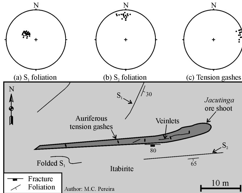
Fig. 10: Geological sketch of the Sump jacutinga orebody (modified by A.R. Cabral after unpublished report by M.C. Pereira, CVRD, 2001). Stereograms (pole to plane, lower hemisphere): (a) main foliation, S_1 ; (b) transposition surface, S_2 ; (c) tension gashes in the jacutinga vein.
