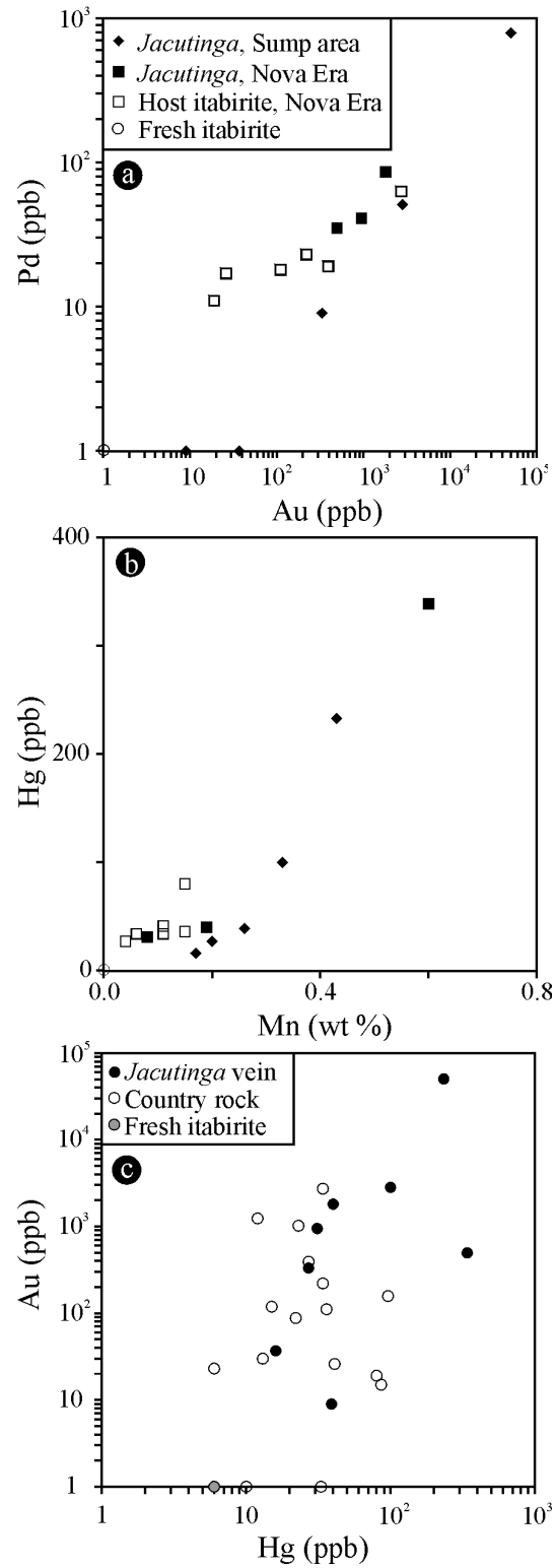
Fig. 27: (a) Pd vs. Au and (b) Hg vs. Mn plots of the bulk-rock chemical analyses in Table 10; legend as in (a). (c) Hg vs. Au plot from data in Tables 10 and 11.
