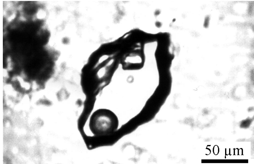
Fig. 25: Primary fluid inclusion in specular hematite with vapour bubble and daughter crystal of unknown composition. Transmitted infrared light, Sump area.
