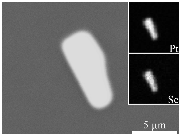
Fig. 40: Crystal of sudovikovite, PtSe 2 , included in vein-related specularite, which grew over a matrix of Cr-magnetite (Y orebody, level 802), and X-ray element-distribution of PtL \alpha and SeK \alpha .
