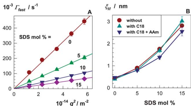
Fig. 1 (A): Relaxation rate of the fast mode ( \Gamma_{fast} ) plotted against q^2 for 0.24 M CTAB-SDS solutions with various SDS contents. Temperature = 35 °C. (B): Hydrodynamic correlation length \xi_H of 0.24 M CTAB-SDS solutions with or without the monomers plotted against the SDS content of the micellar solution.
