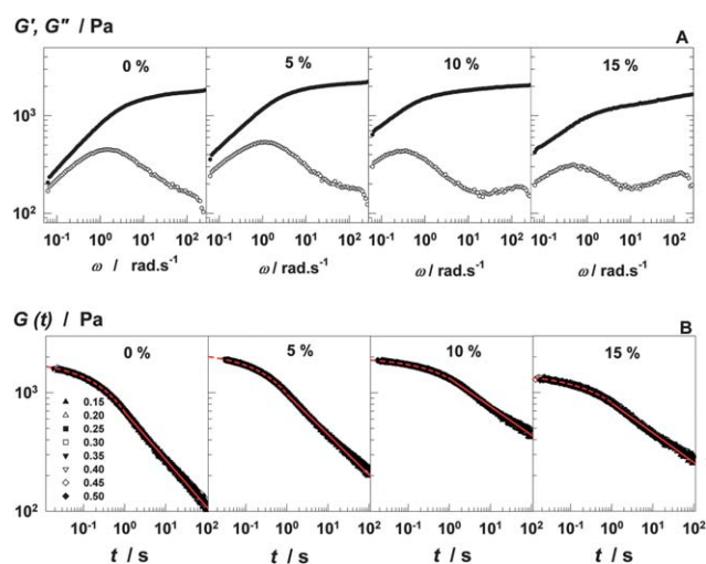
Fig. 4 (A): G' (●) and G'' (○) of gels shown as a function of angular frequency \omega . \gamma_0 = 0.01 . SDS amounts in CTAB-SDS mixtures (in mol%) are indicated. Temperature = 35 °C. (B): The relaxation modulus G(t) of gels as a function of time t for various strains \gamma_0 indicated.
