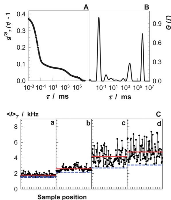
Fig. 3 (A and B): ICF and distribution of relaxation times G(I) obtained with a measurement time of 2 h at \theta = 90^\circ on a gel formed with 15 mol% SDS. Temperature = 35 °C. (C): Variation of \langle I \rangle_T at \theta = 90^\circ with hundred different sample positions for gels formed at 0 (a), 5 (b), 10 (c) and 15 mol% SDS (d). Measurement time per position = 100 s.
