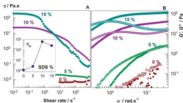
Fig. 6 Flow curves (viscosity vs. shear rate) (A) and frequency-sweeps (B) for the polymer solutions in 0.24 M surfactant solutions with various SDS contents indicated. In (B), G' and G'' are shown by the filled and open symbols, respectively. Polymer concentration = 0.5 w/v%. Inset to (A): specific viscosity \eta_{sp} of polymer solutions as a function of SDS content. Temperature = 35 °C.
