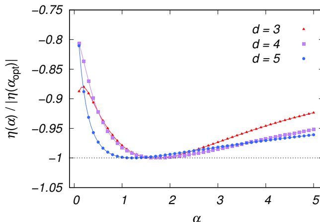
Figure 3. Rescaled anomalous dimension \eta(\alpha)/|\eta(\alpha_{\text{opt}})| shown as a function of \alpha . Different curves correspond to data obtained in d = 3, 4, and 5 dimensions, respectively. The optimal value \alpha_{\text{opt}} for which the critical exponent is least sensitive to changes in the deformation parameter, i.e., \eta'(\alpha = \alpha_{\text{opt}}) = 0 , shifts to larger values as the dimension d is lowered. The displayed values were obtained for a truncation of the scale-dependent effective action \Gamma_k of the type (4, 2, 0) .
