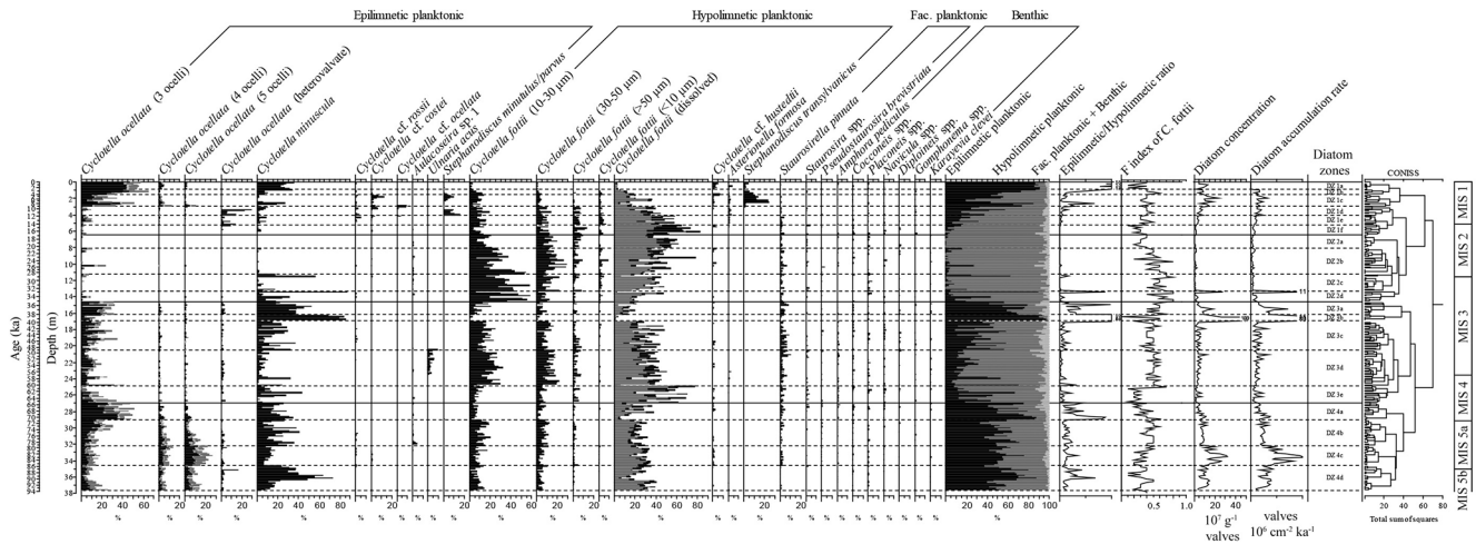
Figure 2. Stratigraphic diatom diagram showing species with > 2% abundance in Lake Ohrid DEEP site core 5045-1, F index of Cyclotella fottii , diatom concentrations ( [n] valves \times 10^7 g -1 dry sediment) and diatom accumulation rates ( [n] valves \times 10^6 cm -2 ka -1 ). Diatom zone boundaries are defined by CONISS, Marine Isotope Stages (MIS) boundaries after Lisiecki and Raymo (2005).
