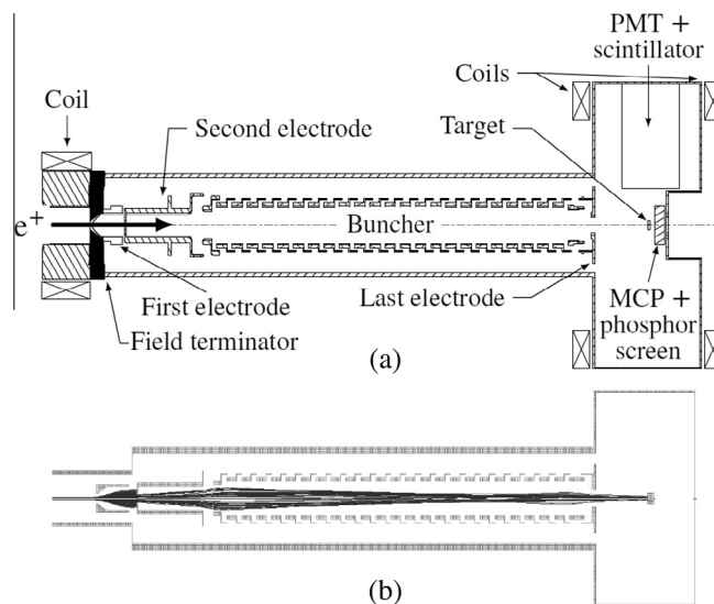
Fig. 3. Sketch of the electrostatic system (a) and simulation of positron bunching and focusing from the end of magnetic section to the target performed with the SIMION® 8 code (b).
