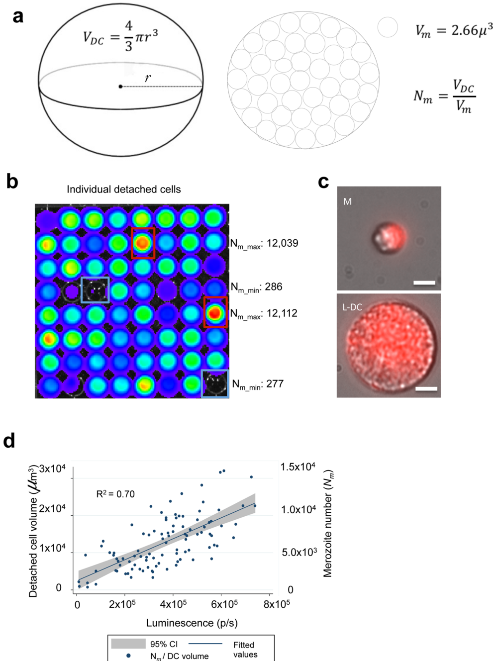
Fig. 5 NanoLuc imaging of P. berghei detached cells allows calculation of merozoite numbers. a Schematic representation of a detached cell. The calculation of merozoite numbers within a detached cell is derived from measurement of the detached cell volume. b Representative bioluminescent image of 64 individual detached cells. c Fluorescence images of 2 types of detached cell accounting for variability in luminescent measurements. The top panel shows a merozoite (M) with even distribution of merozoites within the cell body. The bottom panel shows a large detached cell (L-DC) with even distribution of merozoites within the cell body. Scale bar corresponds to 10 \mu\text{m} . d Scatter plot showing significant correlation of detached cell volumes and merozoite numbers ( y -axis), with and PbNLuc luminescence ( x -axis). 100 individual detached cells symbolizing successful completion of PbNLuc liver infections (represented by each dot) were detected by mCherry-based fluorescence microscopy, imaged, and then individually captured and lysed for luminescence imaging. The radius of the detached cell was measured, and the volume of the detached cell thereby estimated as described in (a) [luminescence measured in photons per second (p/s)]
