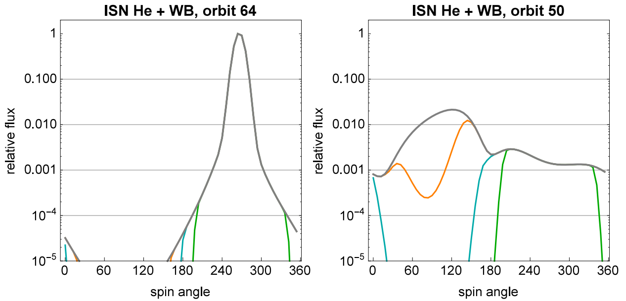
Fig. 10.— He flux scaled to the maximum flux for orbits 64 (the spring peak orbit, left panel) and 50 (the fall peak orbit, right panel) for energy cutoff 0 (gray), 10 eV (orange), 19 eV (blue), and 38 eV (green), simulated assuming the ISN He and Warm Breeze Maxwellian population in front of the heliopause.
