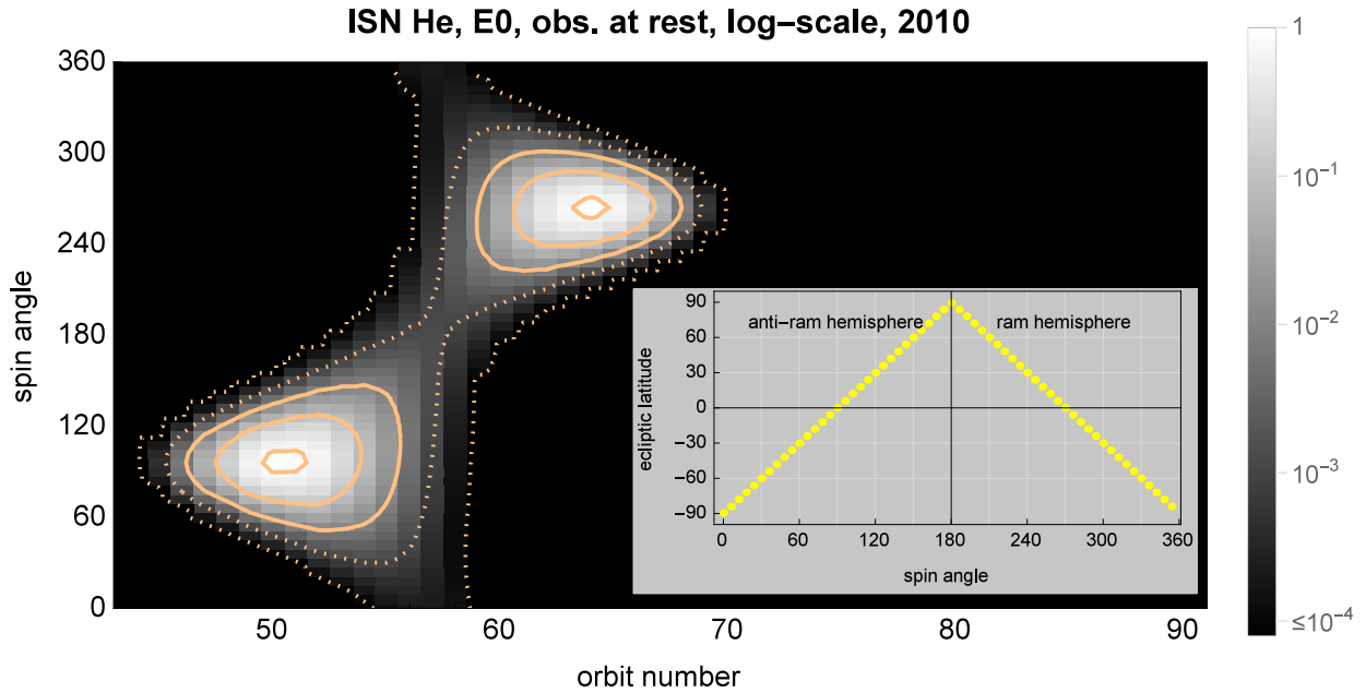
Fig. 2.— Simulated full-sky map of the ISN He flux (single Maxwell–Boltzmann population) as it would be seen by a virtual IBEX -Lo located at ecliptic longitudes corresponding to the longitudes of IBEX orbits 43 through 91 (2009-2010 to August 30), with spin axis oriented identically as it was in reality, but at rest in the Sun frame. The flux is shown in the logarithmic scale and rescaled so that the peak value is equal to 1. The solid isocontour lines show 0.8, 10^{-1} , and 10^{-2} of the peak value, and the two broken isocontours correspond to 10^{-3} and 10^{-4} of the maximum flux, i.e., the isocontours cover (with some excess) the whole dynamical range of IBEX -Lo data. The map is shown in the spacecraft reference system. The figure is built with vertical strips composed of 6^\circ -bins in spin-angle. Those strips correspond to the flux calculated for individual orbits for the full range of spin-angles, i.e., from 0^\circ to 360^\circ , tabulated for the center of the actual 6^\circ -bins of IBEX -Lo. The approximate correspondence between spin-angles and ecliptic latitude, in the convention adopted in this paper, is shown in the inset. A similar format is used in other sky maps presented in the paper.
