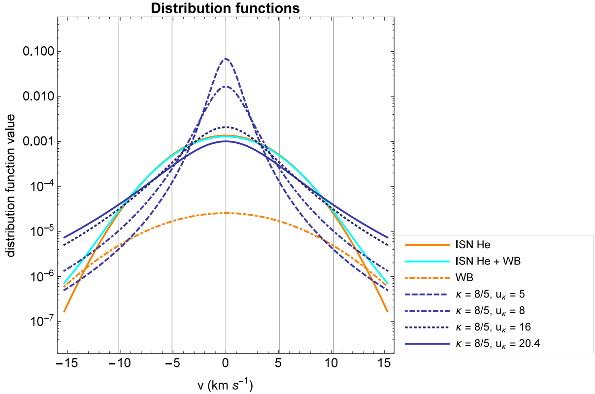
Fig. 4.— Distribution functions used in this study: Maxwell–Boltzmann (Equation 1) with thermal speed value u_{\text{lim}} = 5.06 \text{ km s}^{-1} , characteristic for temperature 6165 K, as found by Bzowski et al. (2012) for ISN He population, Maxwell–Boltzmann with the thermal speed characteristic for the Warm Breeze temperature of 15068 K, as found by Kubiak et al. (2014). The density is scaled to maintain the proportions between the shown cases. The kappa distribution functions come from Equation 2 for \kappa = 8/5 with different u_\kappa given in \text{km s}^{-1} . Note that the plot for the superposition of the ISN He + Warm Breeze case is only an approximation because in reality the mean velocity vector of the Warm Breeze in the reference frame co-moving with the ISN He population is not zero. Thus, only the widths and absolute densities of the ISN He and WB populations can be compared in this figure.
