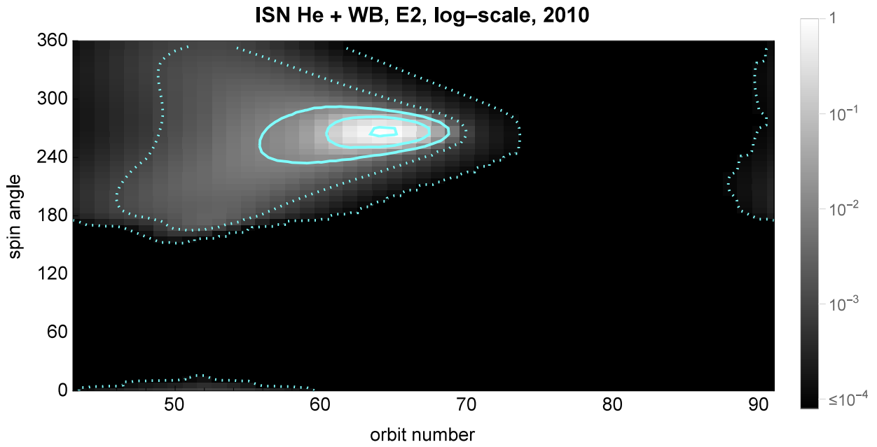
Fig. 12.— Simulated sky map of helium flux (the ISN He + Warm Breeze case), equivalent to Figure 7, calculated with the energy threshold of 19 eV.
