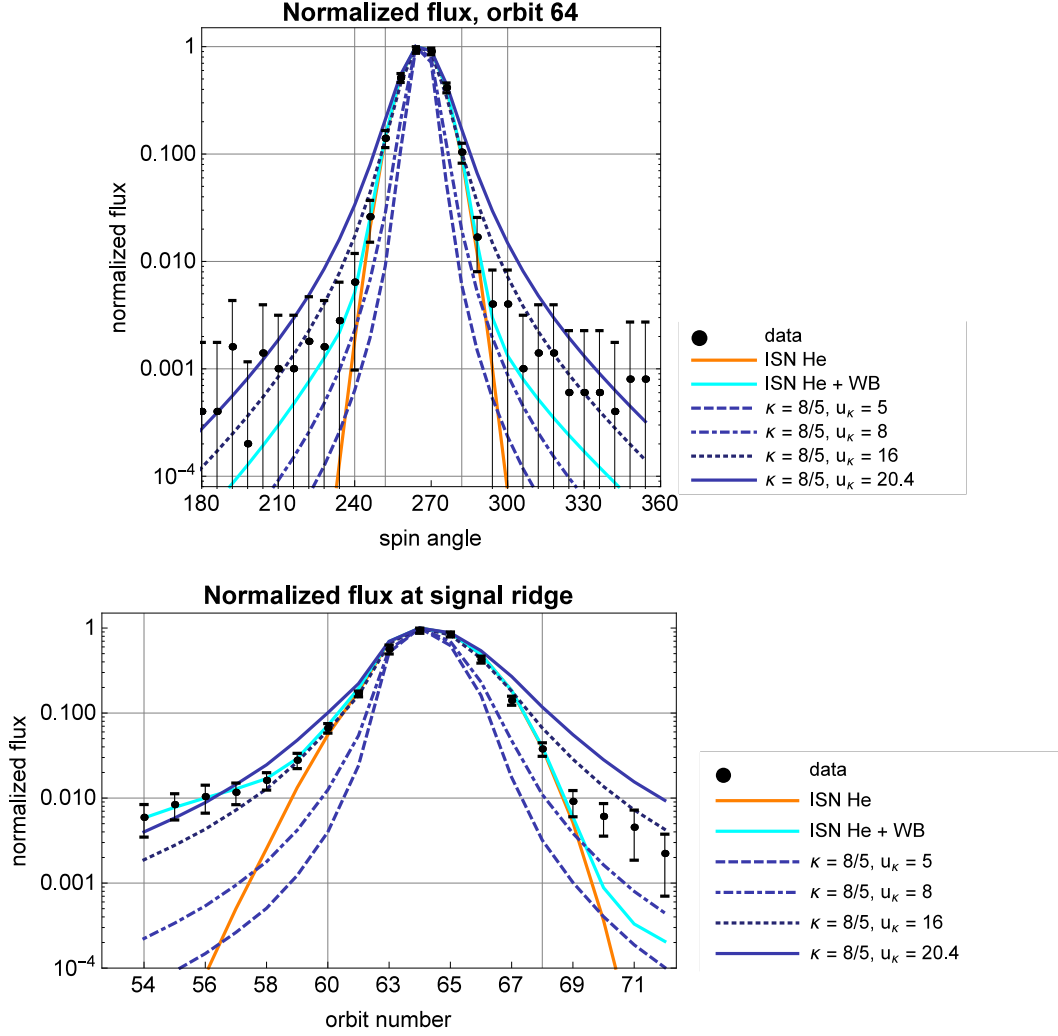
Fig. 15.— Two cuts through the sky maps discussed in the paper. The upper panel shows the cut along the spin angle for orbit 64 (spring peak, \lambda_E \sim 136^\circ , the vertical direction in the sky map plots) and the lower panel shows the cut along a fixed spin angle value of 264^\circ , equal to the spin angle of the maximum flux in orbit 64. The colors are explained in the legend, and u_\kappa is given in \text{km s}^{-1} . The innermost vertical grid lines in the upper panel mark the data points taken by Bzowski et al. (2012) for ISN He analysis, and the outermost grid lines the data points used by Kubiak et al. (2014) for the Warm Breeze analysis. The extreme left and right vertical grid lines for orbits 54 and 68, respectively, in the lower panel mark the first and the last orbit used by Kubiak et al. (2014) for the Warm Breeze analysis, while the grid lines 61 and 68 span the subset of orbits used by Bzowski et al. (2012) for ISN He analysis.
