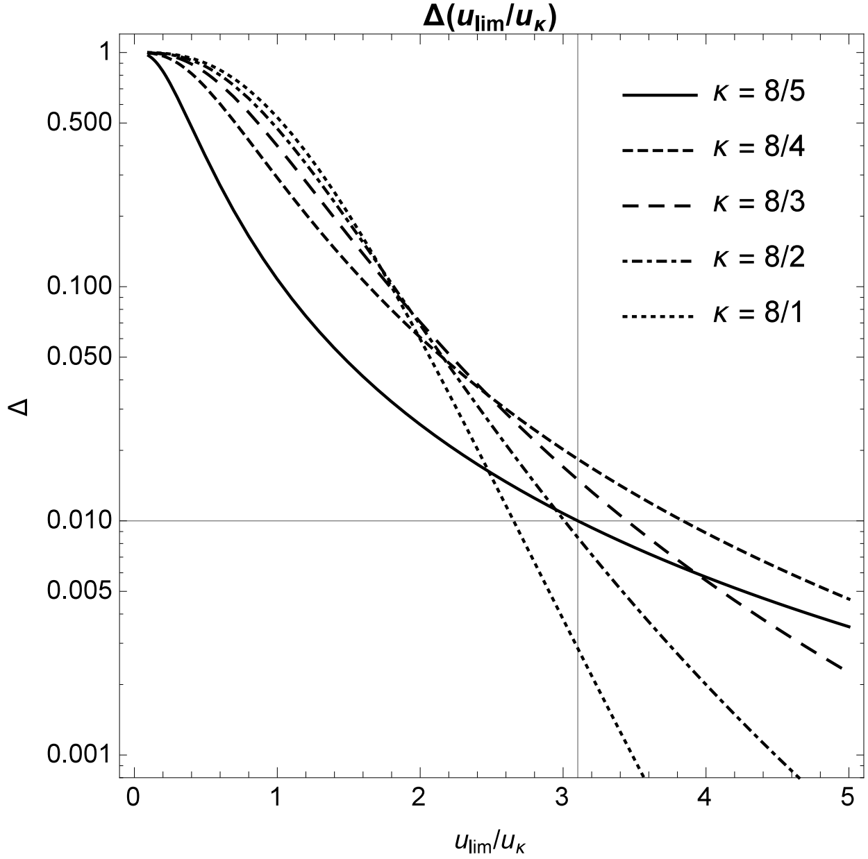
Fig. 3.— Fraction \Delta(u_{\text{lim}}/u_{\kappa}) of the total density left out from integration of the kappa distribution function defined in Equation 2 from 0 to the upper boundary u_{\text{lim}} . The crosshairs mark the u_{\text{lim}}/u_{\kappa} value for \kappa = 8/5 for the \Delta(u_{\text{lim}}/u_{\kappa}) = 0.01 adopted in the paper.
