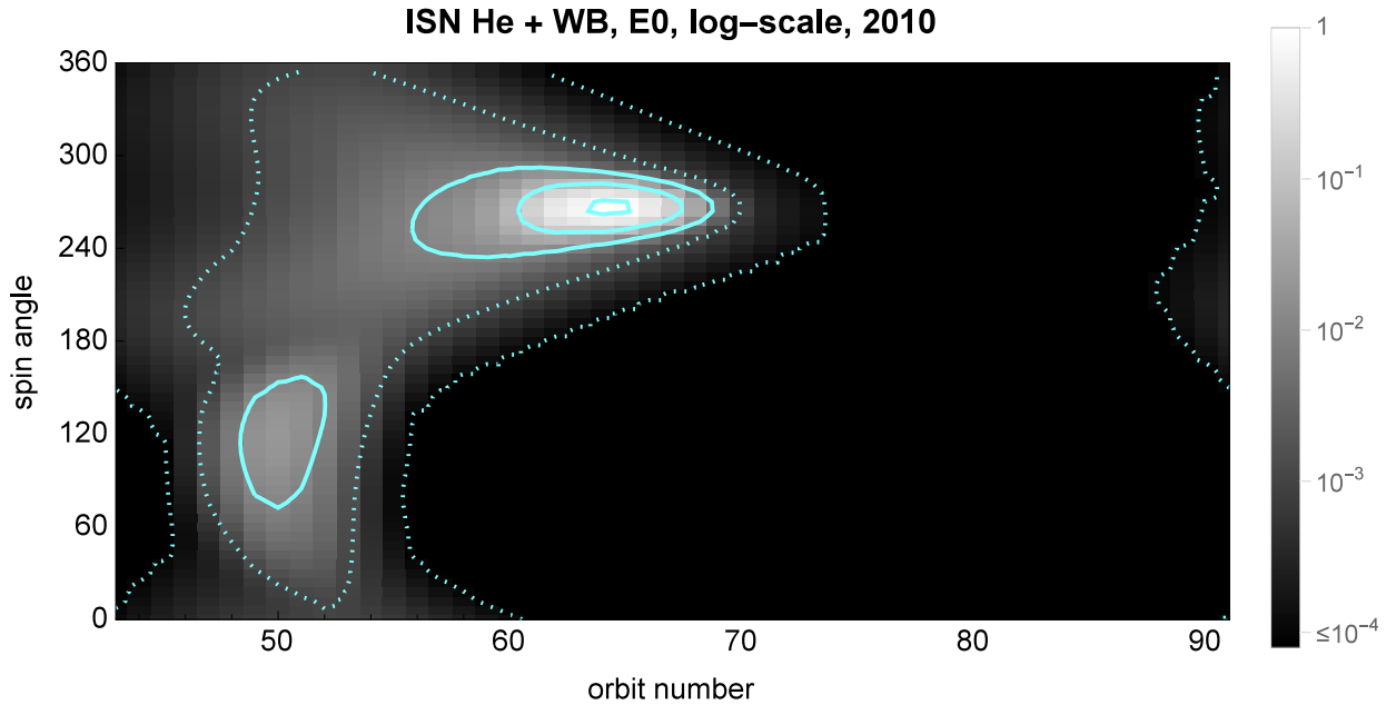
Fig. 7.— Full-sky map of interstellar helium flux, simulated as a superposition of the flux of the ISN He primary population, shown in Figure 5, and of the Warm Breeze. The figure format is identical as to that in Figure 5.
