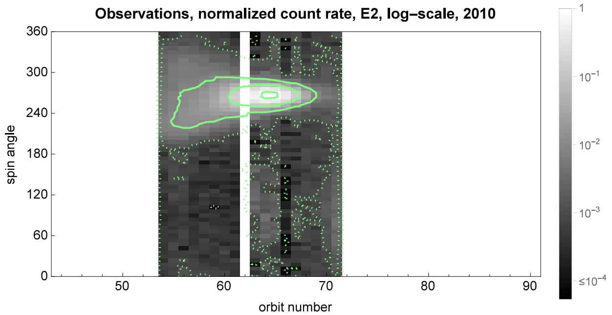
Fig. 9.— Observations from energy step 2 of IBEX -Lo taken in orbits 54 through 72. The grayscale shows the logarithm of the count rate normalized to the peak count rate registered during the 2010 ISN gas observations campaign (orbit 64). The isocontour lines mark the intensities of 0.8, 10^{-1} , 10^{-2} (solid lines), 10^{-3} and 10^{-4} of the peak intensity (broken line). Data from orbit 62 are missing (white block).
