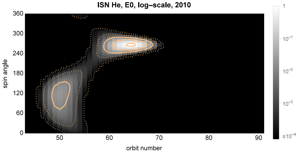
Fig. 5.— Full-sky map of ISN He flux for the single Maxwell-Boltzmann distribution (Equation 1) of the primary ISN He population as it would be seen by IBEX-Lo , if its energy sensitivity was independent of energy. The thermal speed u_{\text{lim}} was \sim 5 \text{ km s}^{-1} . The map is constructed of vertical strips corresponding to the flux observed on subsequent orbits. The strips are located side by side, in chronological order. The flux is scaled to the global maximum (spring peak) and presented in the logarithm scale. The color ovals are the flux isocontours lines located at 0.8, 10^{-1} , 10^{-2} (solid lines), and 10^{-3} and 10^{-4} of the spring peak value (broken lines). The flux distribution on the sky for the values lower than 10^{-4} of the peak value are drawn as totally black.
