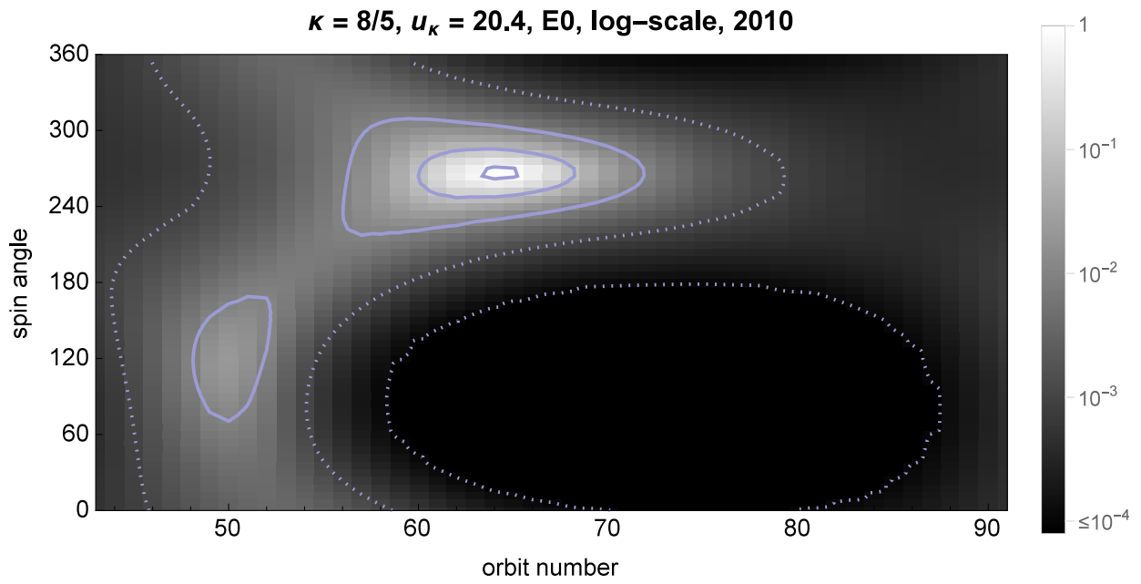
Fig. 8.— Full-sky map of the ISN He population simulated, assuming that the distribution function of ISN He gas in front of the heliopause is given by the kappa function, with \kappa = 8/5 and the extreme case of the reference speed u_\kappa = 20.4 \text{ km s}^{-1} . The figure format is identical as to that in Figure 5.
