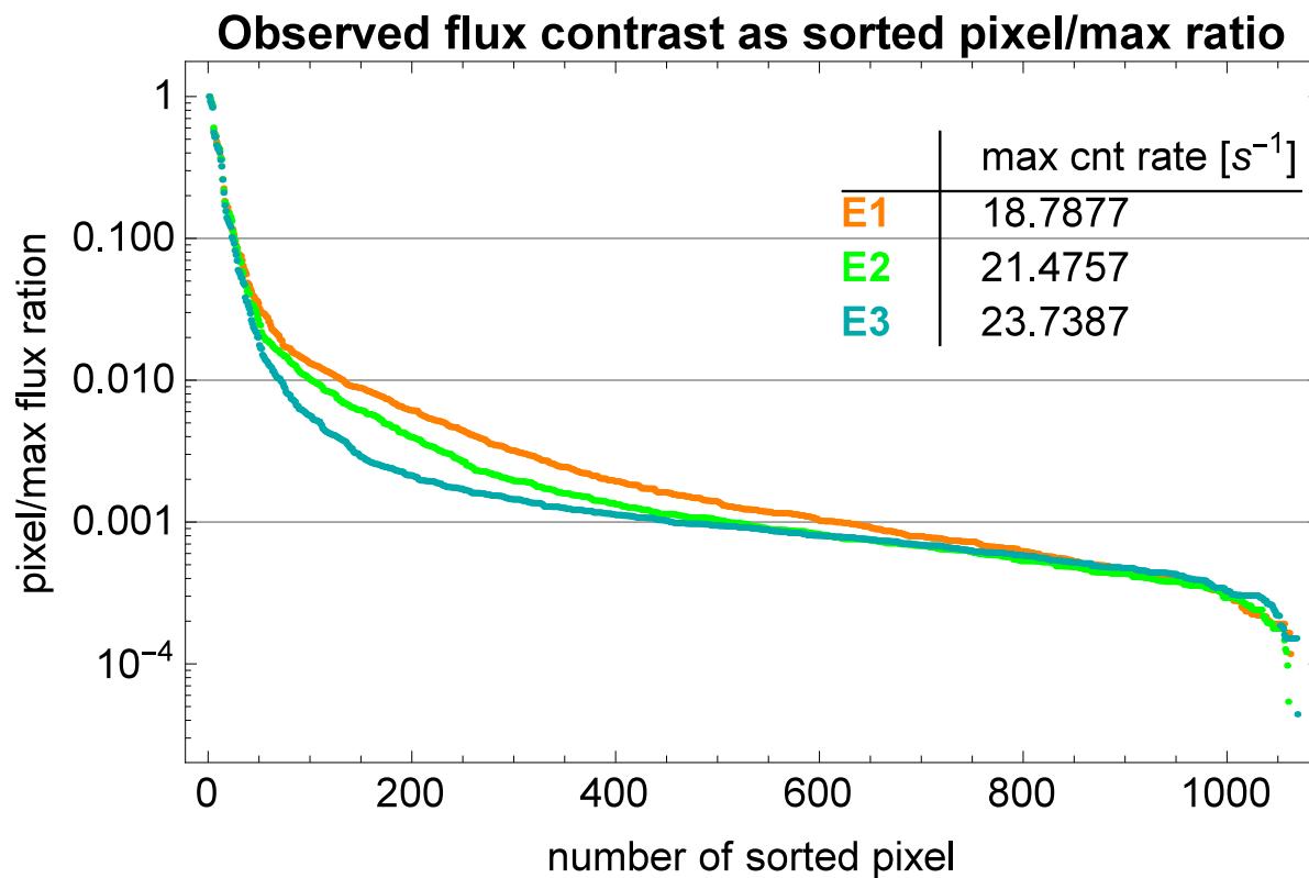
Fig. 1.— Ratios of count rates in individual IBEX -Lo 6^\circ -bins (pixels) to the maximum count rate for a given energy step, sorted in increasing order, for all 6^\circ -pixels in energy steps 1 (orange), 2 (green), and 3 (blue) from orbits 54 through 72, shown as an example to illustrate the high dynamic range of IBEX -Lo observations. The inset table shows the maximum count rates in all three energy steps, observed during the 2009/2010 ISN observation season. There are 18 \times 60 = 1080 bins for one energy step. The bins from E2 constitute pixels of the data map shown further on in Figure 9. The background has not been subtracted.
