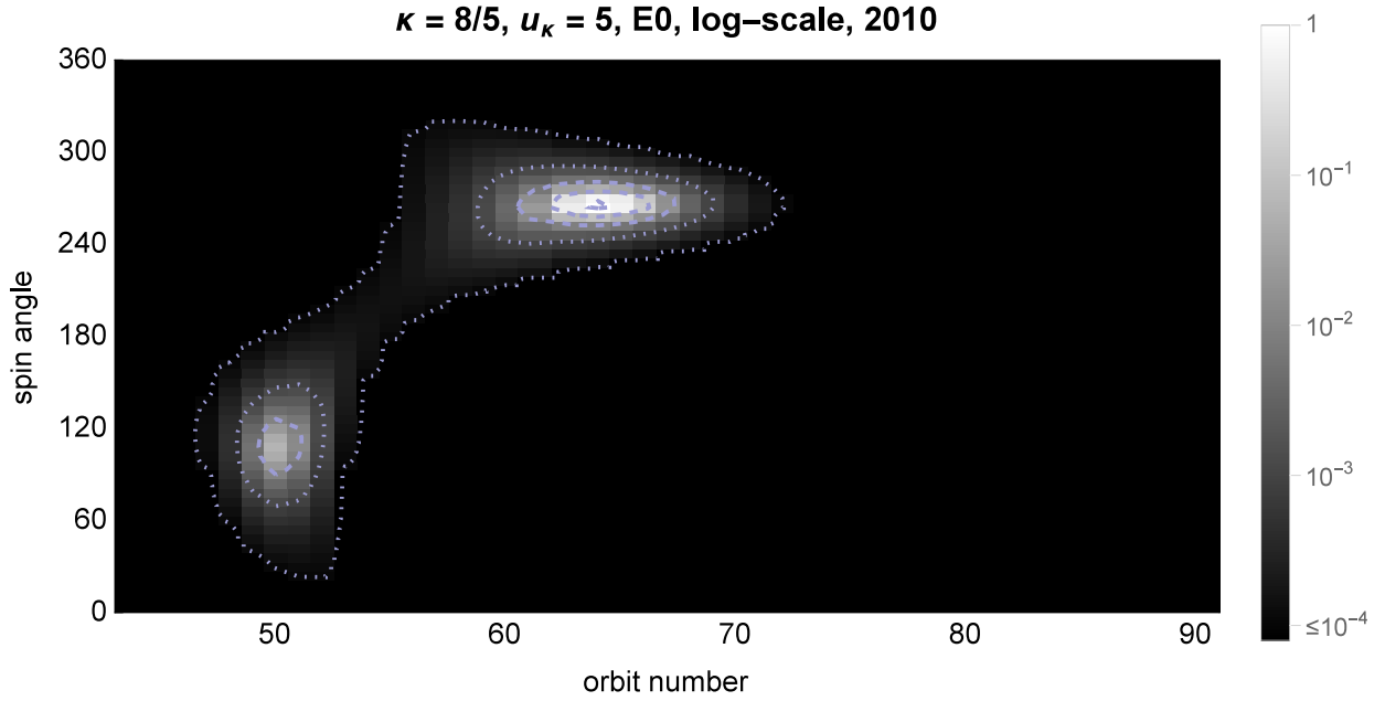
Fig. 6.— Full-sky map of ISN He flux for the narrow kappa distribution assumed in front of the heliopause, with \kappa = 8/5 and the reference speed u_\kappa = 5 \text{ km s}^{-1} . The figure format is identical as in Figure 5.
