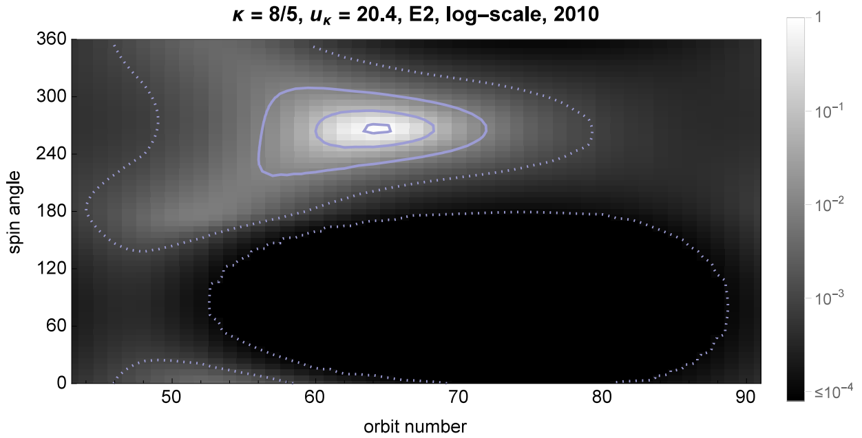
Fig. 13.— Simulated sky map of ISN He flux ( \kappa = 8/5, u_\kappa = 20.4 \text{ km s}^{-1} ), equivalent to Figure 8, calculated with the energy threshold of 19 eV.
