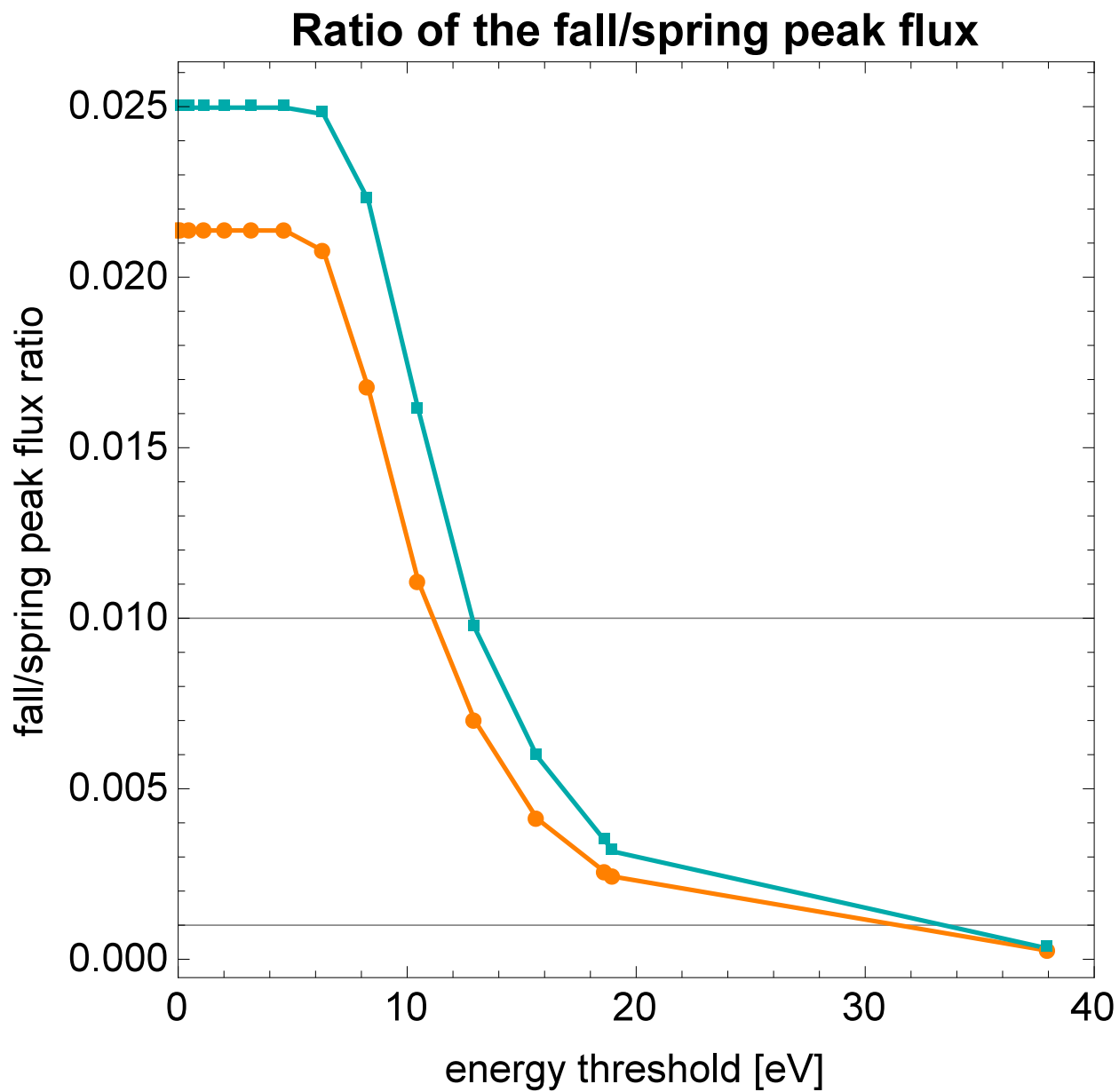
Fig. 14.— Ratios of the fluxes in the highest pixels in the fall and spring peaks for the 2009/2010 (orange) and 2013/2014 (blue) ISN He observation seasons, shown as a function of the energy cutoff, for the single-Maxwellian distribution function of ISN He. The horizontal bars correspond to the 10^{-3} and 10^{-2} isocontours shown in Figure 5.
