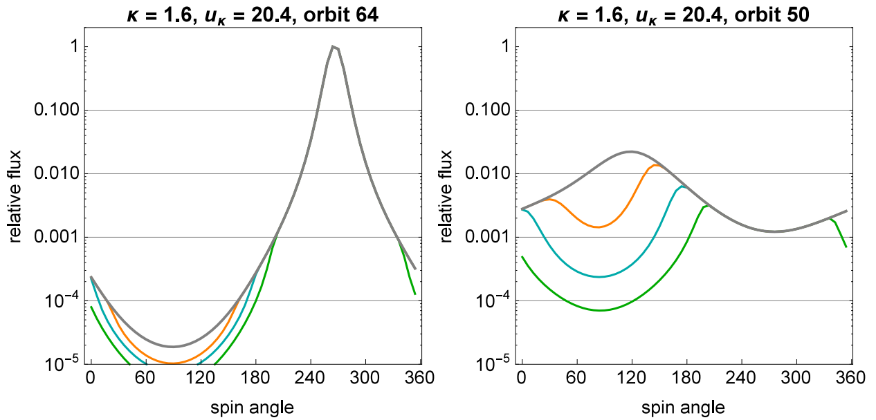
Fig. 11.— He flux as in Figure 10, calculated assuming a kappa population in front of the heliopause with \kappa = 8/5 and reference speed u_\kappa = 20.4 \text{ km s}^{-1} . Note the profound difference between the signal in the anti-ram hemisphere, calculated for four different energy thresholds for the case of kappa function, presented in the right panel of this figure, with the signal simulated for identical energy thresholds for the case of the Maxwellian ISN He + Warm Breeze, shown in the right panel of Figure 10.
