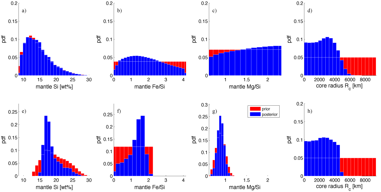
Fig. 14. Sampled 1D marginal posterior distributions for Kepler-36b, case A (a-d) and B (e-h): prior (red) and posterior (blue) of model parameters: (a,e) mantle Si-content \text{Si}_{\odot} , (b,f) mantle \text{Fe}/\text{Si}_{\odot} , (c,g) mantle \text{Mg}/\text{Si}_{\odot} , and (d,h) core radius R_c . Data uncertainties are \sigma_{\text{Fe}/\text{Si}_{\odot}} = 10\% , \sigma_R = 2\% , and \sigma_M = 7\% .
