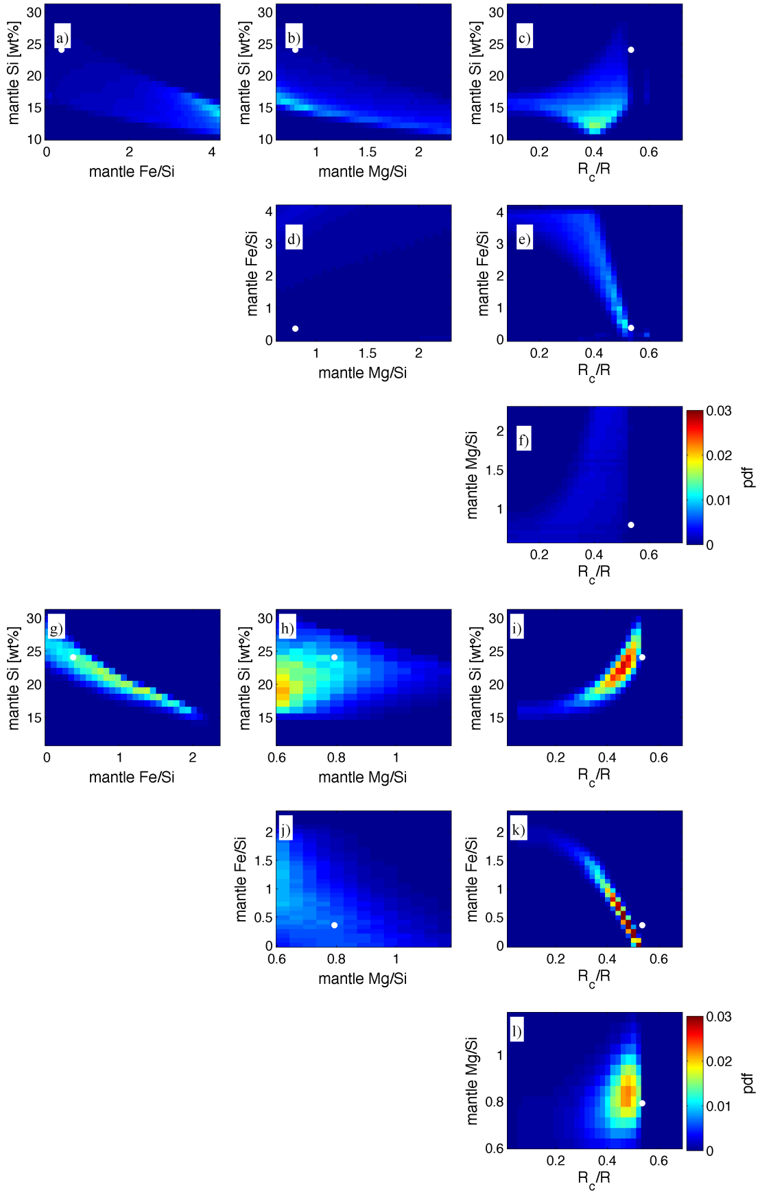
Fig. 5. Sampled 2D marginal posterior distributions for the Earth (case A: plots a–f and case B: plots g–l) showing correlation between parameters \text{Si}_{\odot} , \text{Fe}/\text{Si}_{\odot} , \text{Mg}/\text{Si}_{\odot} , and core radius R_c (corresponding to Figure 4). Independent estimates (Table 2) are marked in white.
