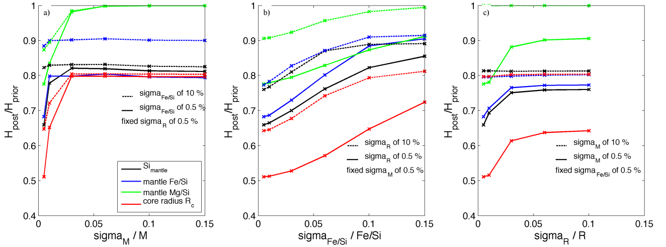
Fig. 16. Summary of information content for an Earth-sized body ( M = 1M_E , R = 1R_E ): Relative Shannon measure as a function of (a) \sigma_M while fixing \sigma_R at 0.5% (b) \sigma_{\text{Fe}/\text{Si}_\odot} while fixing \sigma_M at 0.5% (c) \sigma_R while fixing \sigma_{\text{Fe}/\text{Si}_\odot} at 0.5%.
