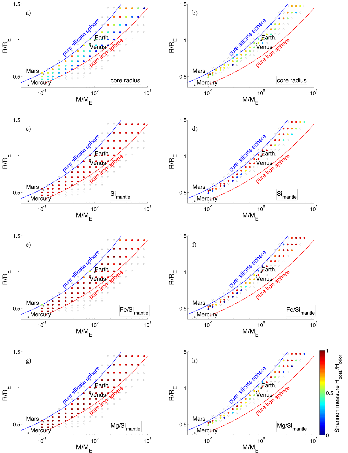
Fig. 12. Relative Shannon entropy measure H_{\text{posterior}}/H_{\text{prior}} of model parameters plotted for the range of synthetic rocky planets that fit a given Article number, page 6 of 19, and M , R , and \text{Fe}/\text{Si}_\odot (case B, right panels). Model parameters are well constrained for H_{\text{posterior}}/H_{\text{prior}} \rightarrow 0 (blue colors) and not constrained for H_{\text{posterior}}/H_{\text{prior}} \rightarrow 1 (red colors). For case B, variations of H_{\text{posterior}}/H_{\text{prior}} along the grid appear not to be smooth which is due to the poor grid resolution. See also Figure 10.
