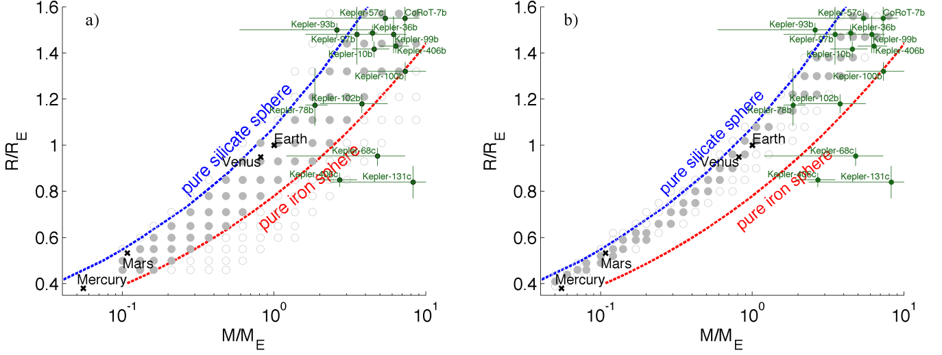
Fig. 13. Confirmed exoplanets plotted against Figure 10: (a) Case A and (b) case B.
