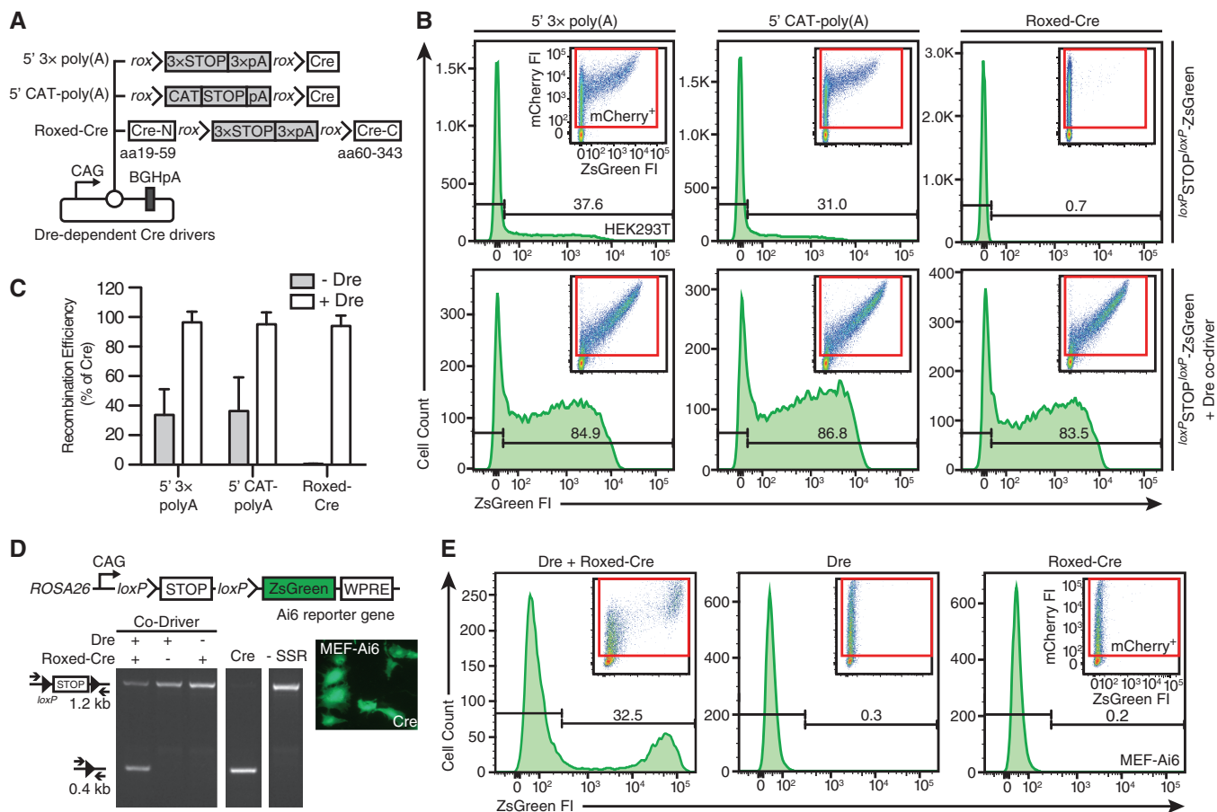
Figure 2. Dre-dependent activation of Cre. (A) Diagram depicting Dre-dependent Cre driver candidates 5' 3× poly(A), 5' CAT-poly(A) and Roxed-Cre with distinct rox-flanked STOP cassette configurations. In the case of Roxed-Cre, the Cre protein-coding sequence is interrupted by a rox-flanked STOP cassette inserted in between the codons of amino acids (aa) 59 and 60. (B) Activity of Cre driver candidates in transfected (mCherry + ) HEK293T is detected using a ZsGreen reporter plasmid. Representative flow plots 24h after transfection of HEK293T cells with a loxP-flanked ZsGreen reporter, Cre-Driver candidates and either omitting (top row) or adding (bottom row) Dre. (C) Quantification of recombination activity of Cre driver candidates with or without Dre Co-Driver. Bars represent the percentage of transfected cells showing recombination activity. Average data of three independent experiments are shown with standard deviation and normalized to 100% Cre average recombination efficiency. (D) MEFs derived from hemizygous Ai6 reporter mice (MEF-Ai6) express ZsGreen from the single copy Ai6 transgene (D top panel; WPRE, woodchuck hepatitis virus post-transcriptional regulatory element) upon Cre recombination (D right panel; fluorescence microscopic image of MEF-Ai6 72h after transfection with Cre). Combined, but not single transfections of Co-Driver modules Dre and Roxed-Cre result in excision of the loxP-flanked Ai6 STOP cassette, as detected by the presence of a 0.4-kb PCR fragment using primers located upstream and downstream of the STOP cassette (D bottom panel) and expression of ZsGreen, as detected by flow cytometry (E) in MEF-Ai6 72h post-transfection.
