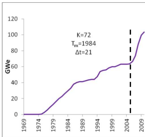
FIGURE C6: CUMULATIVE CAPACITY (US WET FGD) 1969-2010
