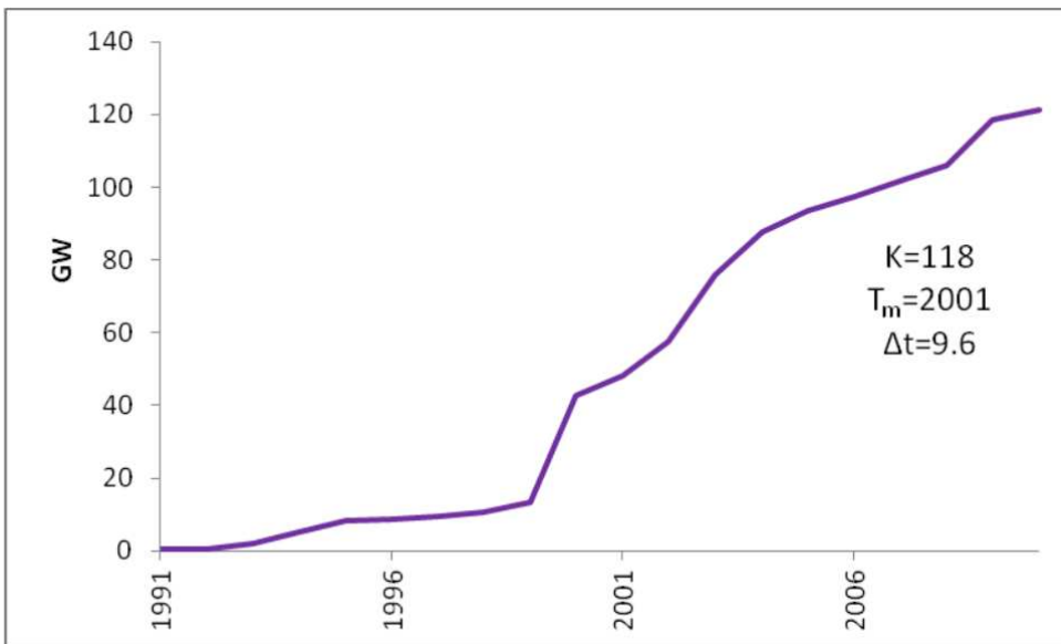
FIGURE C22. SCR CUMULATIVE CAPACITY (US 1991-2010)
