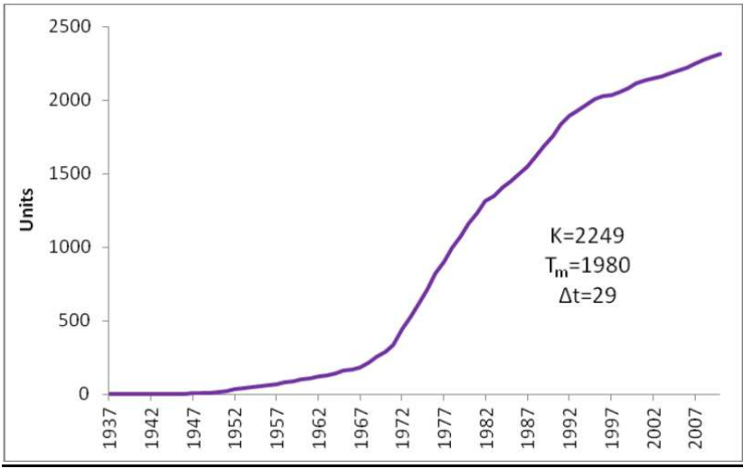
FIGURE C12. TOTAL US FGD CUMULATIVE CAPACITY (1937-2010)
