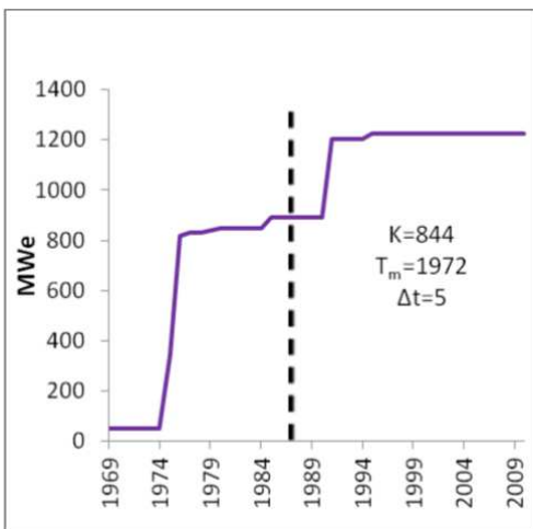
FIGURE C5: MAX UNIT SCALE (US WET FGD) 1969-2010
