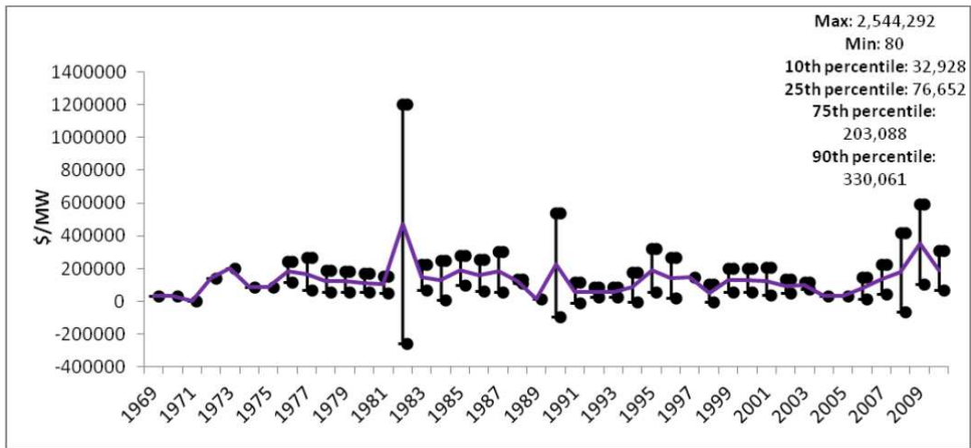
FIGURE D2. COST/MW FOR FGD UNITS (PPI COMMODITY INDEX)
