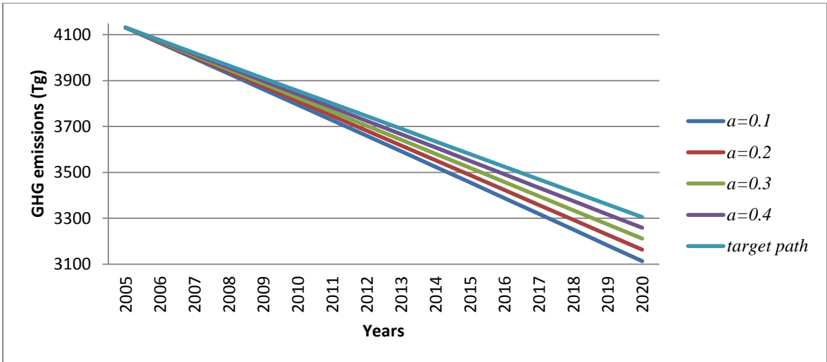
Figure 6. Calculated modified reduction targets CO 2 , N 2 O, CH 4 emissions in CO 2 -equivalent for the EU-15
