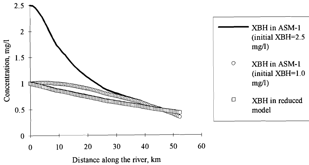
Figure 8. Simulated heterotrophic bacterial biomass longitudinal profiles for ASM-1 and reduced model (not present in QUAL2E).
