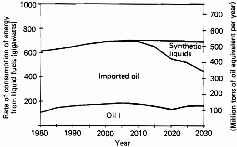
FIGURE 4.12 EC liquid fuel supply in the Coal Case. (See Appendix for cost categories.)
