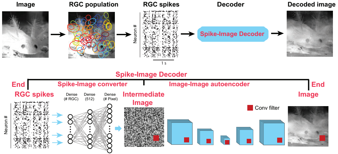
Figure 1: Illustration of the spike-image decoder model. (Top) Workflow of decoding visual scenes. Here a salamander swimming video was presented to a salamander retina to stimulate a firing of spike trains in a population of RGCs. The spikes are used to train the decoder for the given video to reconstruct the visual scene. Receptive fields of ganglion cells are mapped onto the image. Each coloured circle is an outline of receptive field. (Bottom) Spike-image decoder is an end-to-end decoder with two stages: spike-image converter used to map a population of spikes to a pixel-level intermediate image, and image-autoencoder for mapping every pixel to the target pixels in the desired images.
