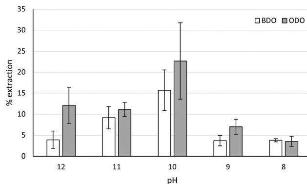
Fig. 4 The % extraction of \text{Cu(II)} from ammoniacal solutions using “BDO” MAL and “ODO” MAL at different pHs and 1 : 1 by weight loading of chelator : \text{Cu(II)} . The pH shown in the graph has been rounded to the nearest whole number for visual clarity. Exact pH values are shown in the ESI.†
