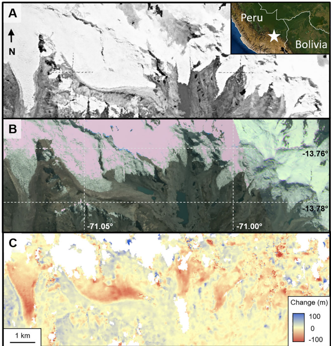
Figure 2. Historic and contemporary images can be used to quantify mass change across the Cordillera Vilcanota, Peru ( -13.76^{\circ}\text{N} , -71.03^{\circ}\text{E} ). (a) KH-9 HEXAGON image from 3rd August 1980, georeferenced and overlain on a DEM generated using HEXIMAP (Maurer and Rupper, 2015); (b) Planet imagery from May 2020 as a visual reference for glacier position today; and (c) DEM differencing the KH-9 HEXAGON elevation model against a TanDEM-X DEM from July 2015. Positive values surrounding the glacier are likely to be due to georeferencing error of the HEXAGON image on very steep slopes.
