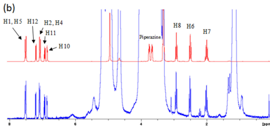
Fig. 3. 1 H NMR spectra (300 MHz) in 5% D 2 O/CD 3 OD of (a) RTC1 (red) and the inclusion complex (blue) and (b) a magnified view of the spectrum.
