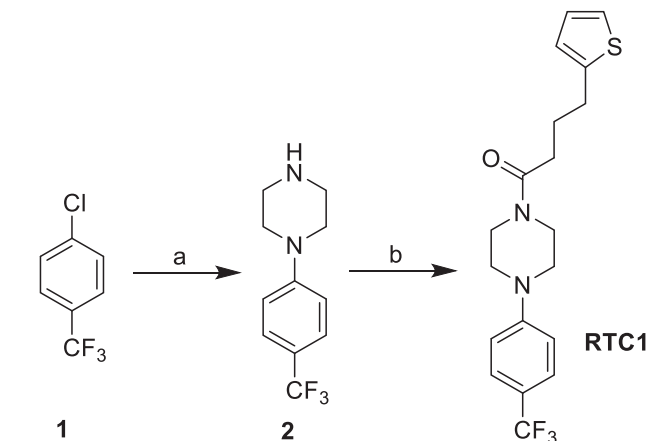
Scheme 1. Synthesis of RTC1. Reagents and conditions: (a) piperazine, NMP, 30 min, 200 °C, MW, 50% yield; (b) 4-(2-thienyl)butyric acid 3 , HOBT, TBTU, NEt 3 , DMF, overnight, rt, 80% yield [9].
