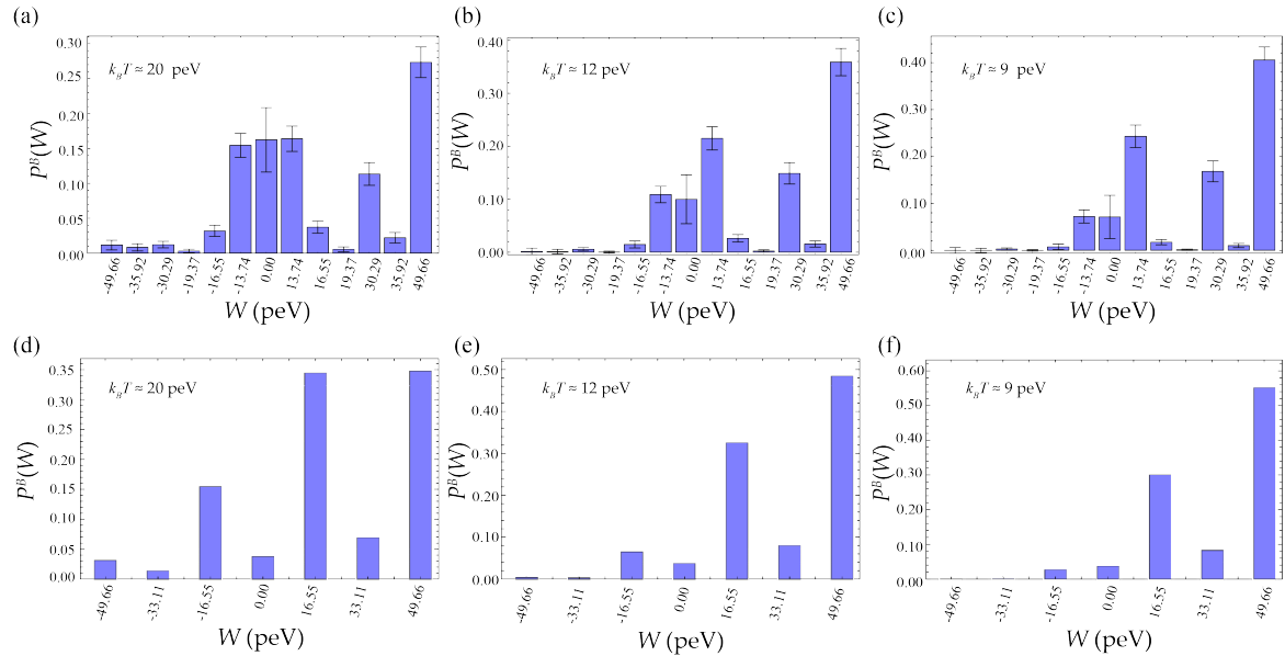
Figure S5. Experimental (a, b, c) and non-interacting theoretical (d, e, f) results for the backward work distribution for the three different initial spin temperatures (a, d) k_B T = 20 \pm 3 \text{ peV} , (b, e) k_B T = 12 \pm 2 \text{ peV} and (c, f) k_B T = 9 \pm 2 \text{ peV} .
