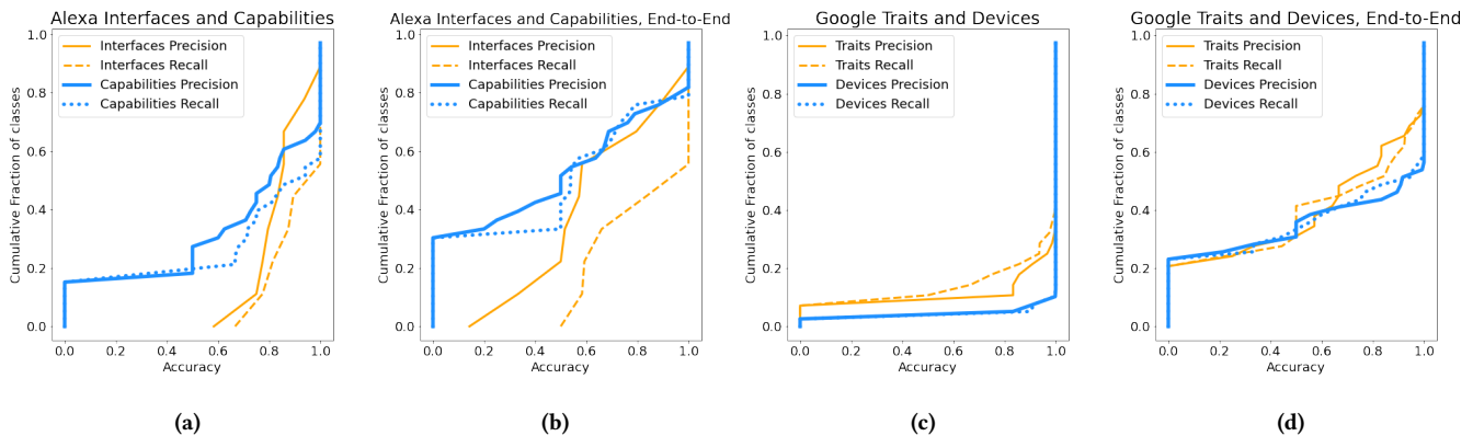
Figure 2: Empirical cumulative density functions (ecdf) of precision and recall for the MobileBERT-quant model. The 25, 50, 75-percentile for precision are (a) 0.77, 0.83 and 0.86 for Alexa interfaces NLU-only, 0.5, 0.80 and 1 for Alexa capabilities, (b) 0.5, 0.57, 0.80 for interfaces end-to-end (E2E), 0.0, 0.5 and 0.79 for capabilities E2E. For Google traits and devices the percentile are (c) 0.95, 1, 1 and (d) 0.11, 0.67, 0.98 for traits E2E and 0.11, 0.90 and 1 for devices E2E. The percentile for recall are (a) 0.81, 0.89 and 1 for interfaces, 0.67, 0.86 and 1 for capabilities, (b) 0.59, 0.83 and 1 for interfaces E2E, 0.0, 0.54 and 0.77 for capabilities E2E, (c) 0.92, 1, 1 for traits and devices and (d) 0.1, 0.75 and 0.97 for traits E2E and 0.83, 1 and 1 for devices E2E.
