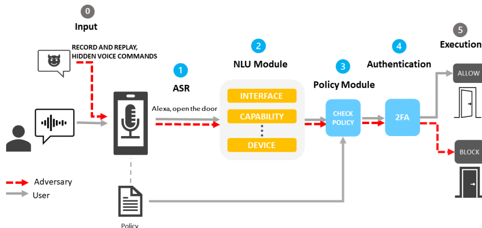
Figure 1: Overview of Sesame, the proposed framework. A spoken command is transcribed by the ASR and classified by the NLU module as a target smart home functionality/device. The Policy module then determines whether the command is to be executed or not and invokes the 2FA and execution steps accordingly.
