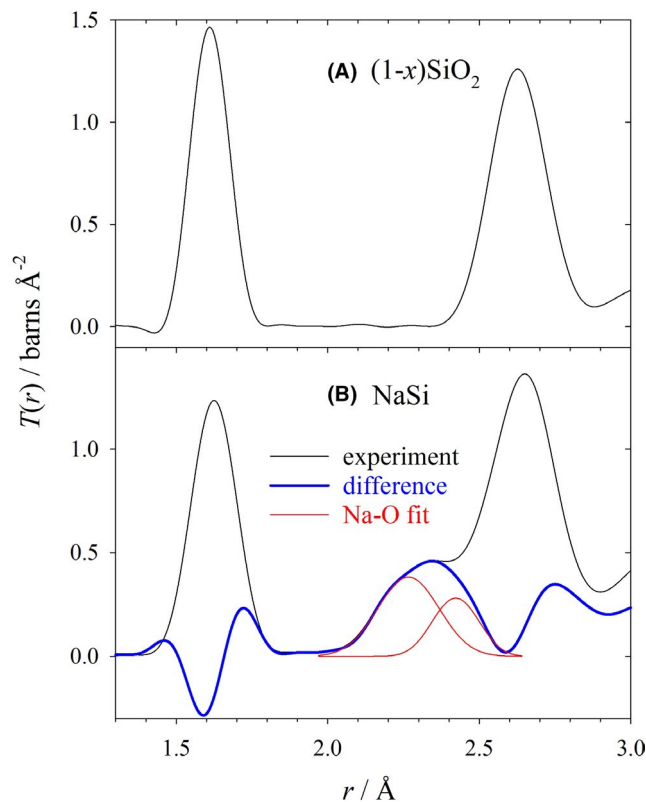
FIGURE 11 Application of the difference method. (A) The total correlation function for pure SiO 2 glass multiplied by a factor (1-x) . (B) The total correlation function (black line) for sodium silicate glass with 42.5 mol% Na 2 O ( x = 0.425 ), the difference, \Delta T(r) , according to Equation 16 (thick blue line), and the two components (red lines) of a two-peak fit to the apparent Na–O contribution to the difference
