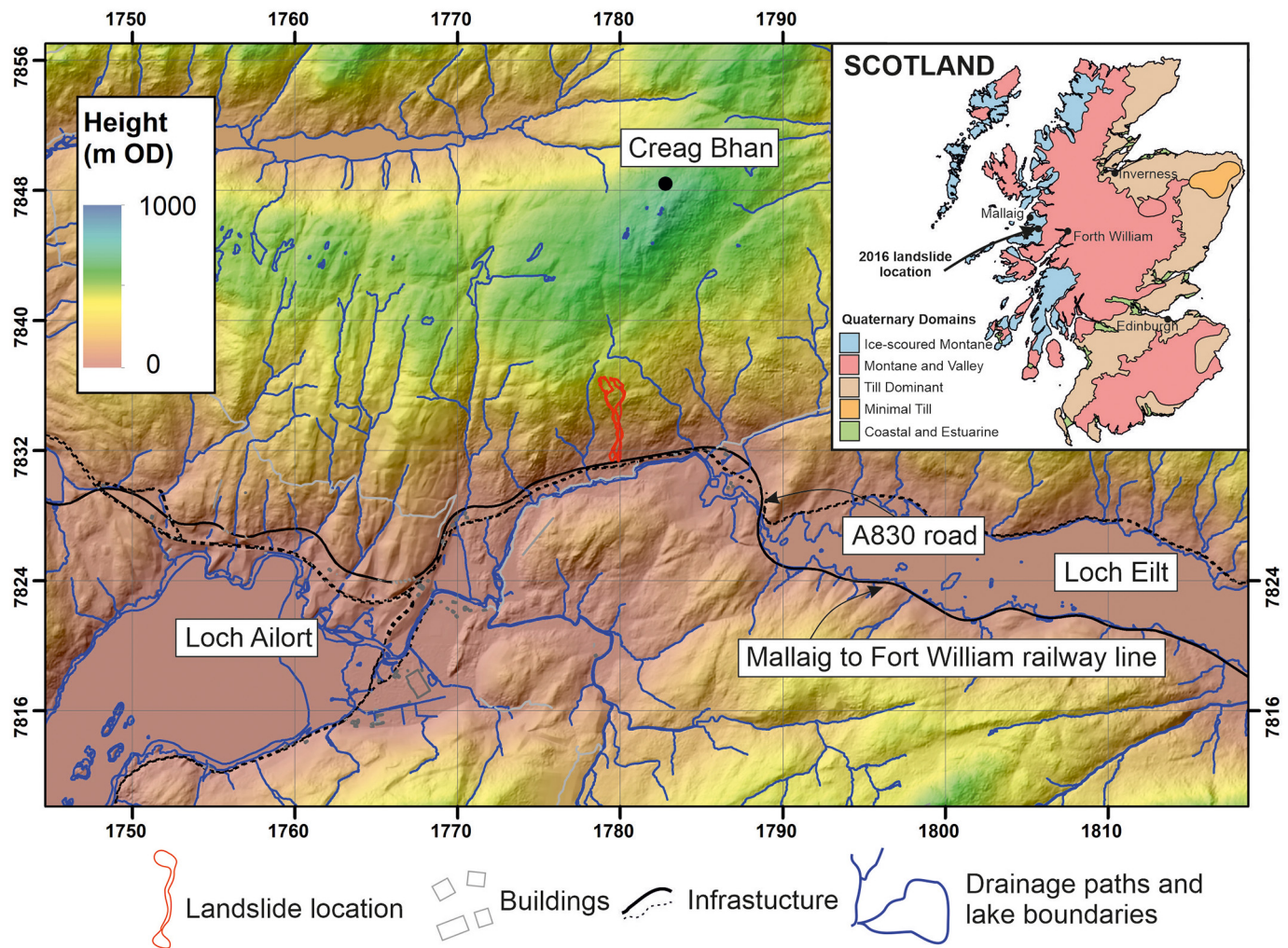
Fig. 1. Overview DEM image of the landslide site between Loch Ailort and Loch Eilt, with local roads and trainline shown. The inset map shows the Quaternary domains (Booth et al., 2015) Derived in part from DTM of Great Britain at 5 m resolution © Bluesky International Limited.
