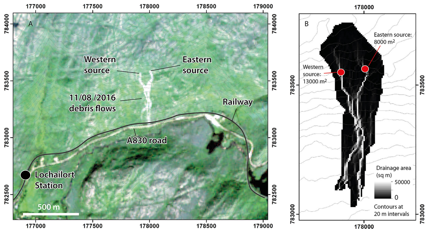
Fig. 3. a) Sentinel 2 image showing two source areas and landslides and b) drainage area for the debris flow catchments. Derived in part from DTM of Great Britain at 5 m resolution © Bluesky International Limited.
