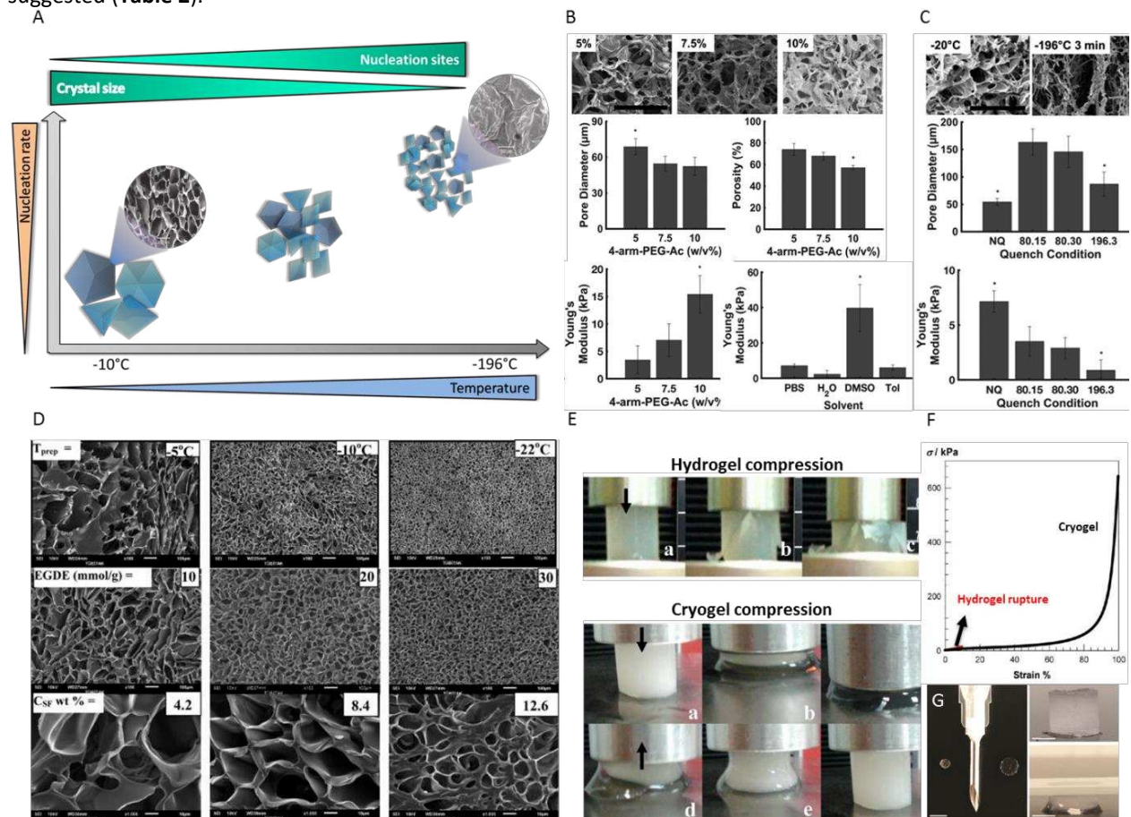
Figure 4: Cryogelation temperature and monomer concentration, effects the pore size and mechanical properties of cryogels. (A) Schematic representation of the ice nucleation process (inserted SEM images adapted with permission from (Kirsebom et al., 2009)). (B, C) Effect of monomer concentration, solvent and quenching on 4-arm PEG-acrylate cryogel properties including pore diameter, porosity and Young's modulus. The scale bar represents 100 μm (reproduced with permission (Bruns et al., 2018)). (D) SEM images of cryogels formed at various temperatures, and monomer concentrations; scale bars = 100 μm (first and second rows) and 10 μm (bottom row) (reproduced with permission (Ak et al., 2013)). (E) Photographs of silk fibroin hydrogels (top) and cryogels (bottom) during the compression tests. (F) Stress-strain curves of these gel samples as the dependence of the nominal stress \sigma on the degree of compression (adapted with permission (Ak et al., 2013)). (G) Photographs of 1.5 and 3 mm diameter cryogels next to a 16G needle, including cryogels before compression (top right) and after (bottom right) compression (scale bars = 3 mm (reproduced with permission (Bruns et al., 2018))).
