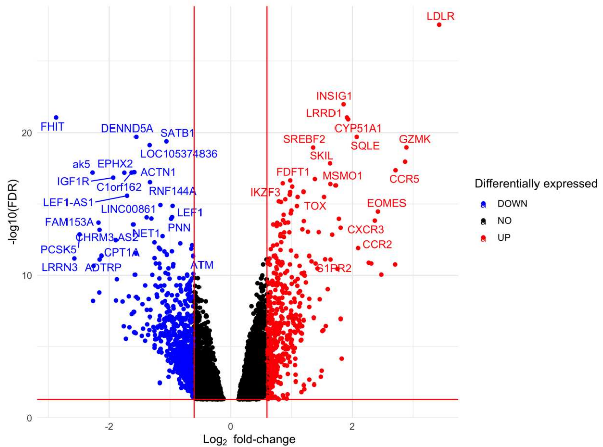
Figure 2. Volcano plot showing differentially expressed genes between CSF and blood CD4 + T-cells in multiple sclerosis. Log 2 fold-change thresholds of +/-0.6 and FDR 0.05 are drawn as red lines for visualisation purposes.
