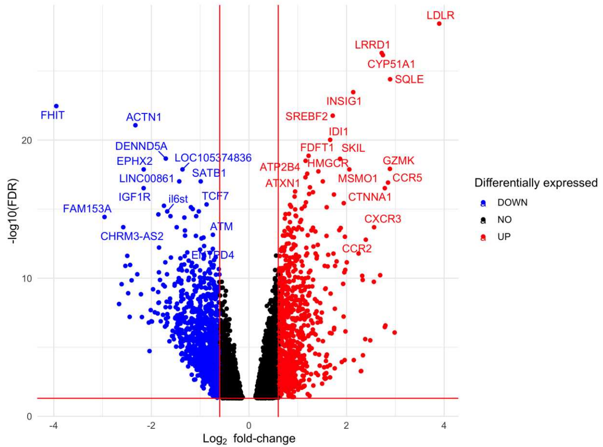
Figure 1. Volcano plot showing differentially expressed genes between CSF and blood CD4 + T-cells in non-inflammatory controls. Log 2 fold-change thresholds of +/-0.6 and FDR 0.05 are drawn as red lines for visualisation purposes.
