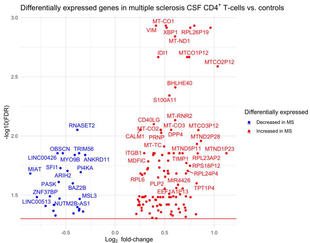
Figure 3. Volcano plot showing differentially expressed genes between multiple sclerosis and non-inflammatory control CSF CD4 + T-cells.
