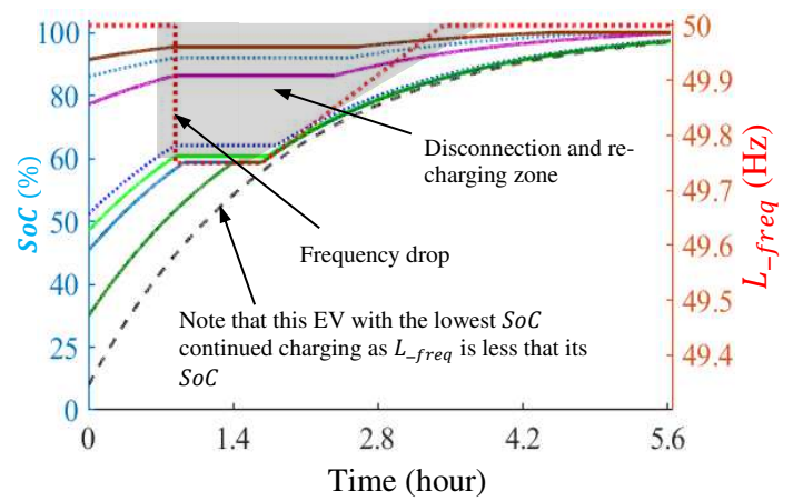
Fig.6 the charging of 10 residential EVs being controlled according to (6) and (7) against a frequency signal
