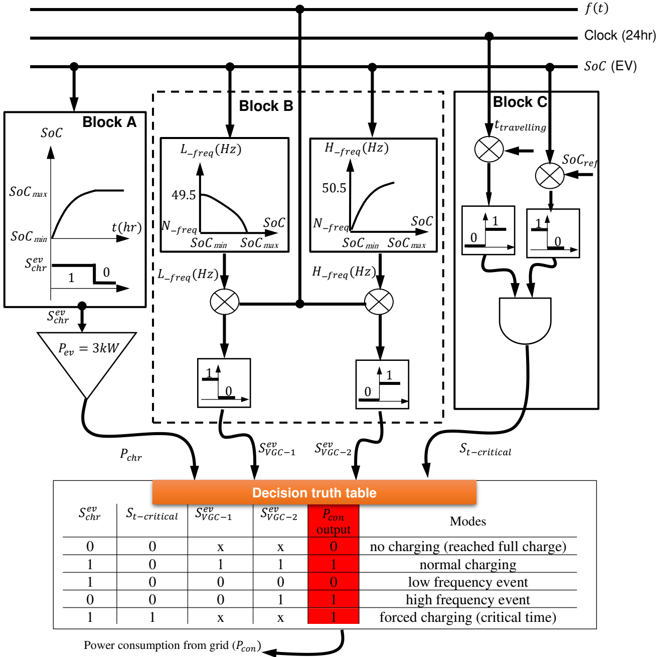
Fig. 3 Framework of EV frequency control system (DVGS controller)
