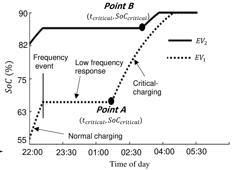
Fig.8 Charging behavior of two EVs with respect to low frequency event and critical time
