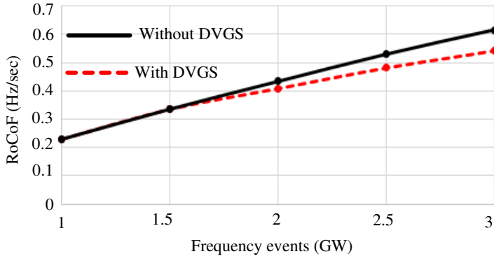
Fig. 14 Rate of change of frequency without DVGS model at 0.05sec following the event
