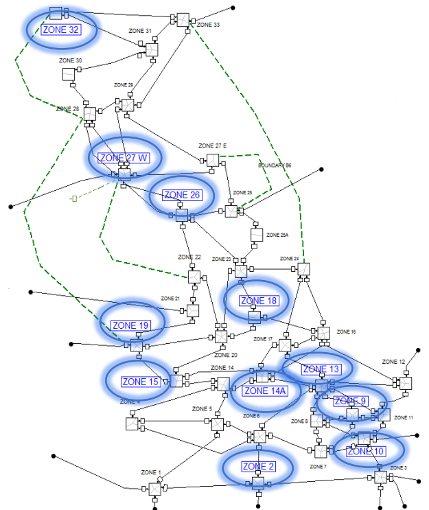
Fig. 9 Reduced GB 36-bus/substation transmission model
