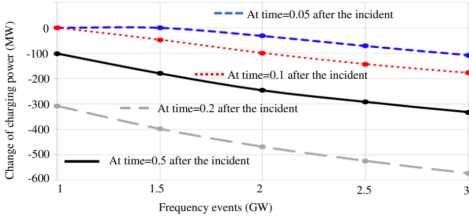
Fig. 18 Change of charging power drawn by EVs in response to frequency event
