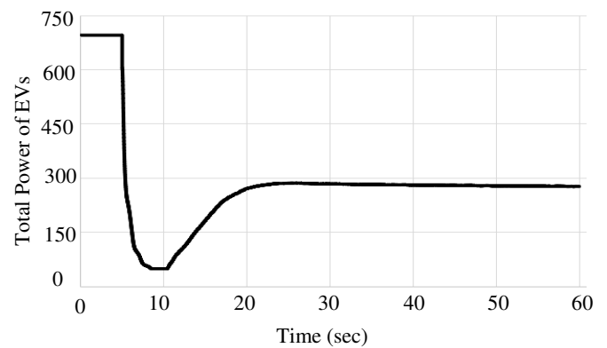
Fig.13 Power EVs at different zones
