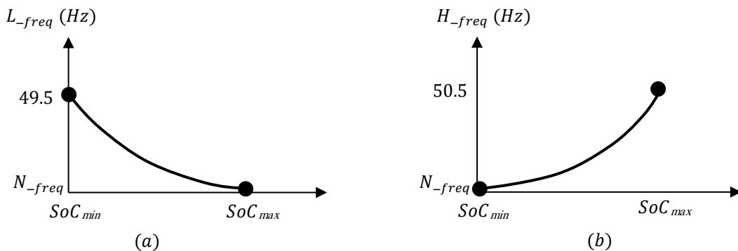
Fig.4 10 Dynamic relationship between the frequency set-points and the SoC (a) L_{freq} set point (b) H_{freq} set-point.
