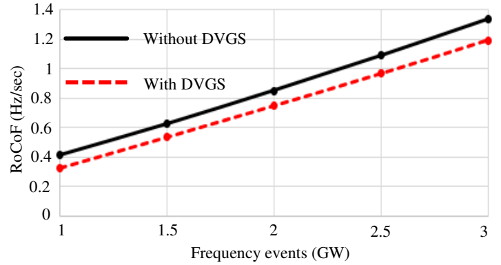
Fig. 17 Rate of change of frequency without DVGS model at 0.5sec following the event
