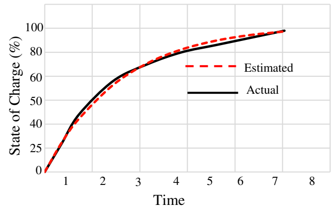
Fig. 2 Charging profile for lead acid battery
