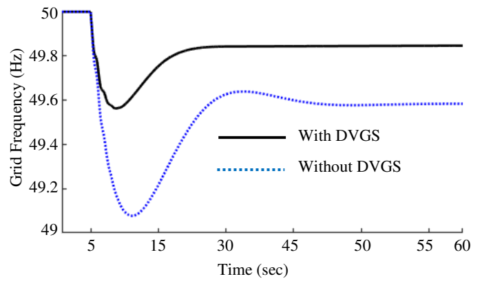
Fig.11 Variation of frequency after generation loss
