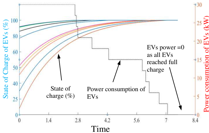
Fig.5 10 residential EVs being charged and their power consumption without frequency event
