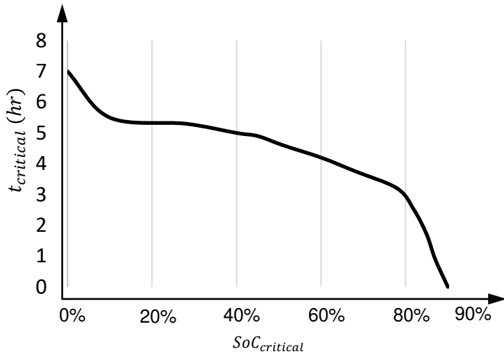
Fig.7 relationship between the t_{critical} and SoC
