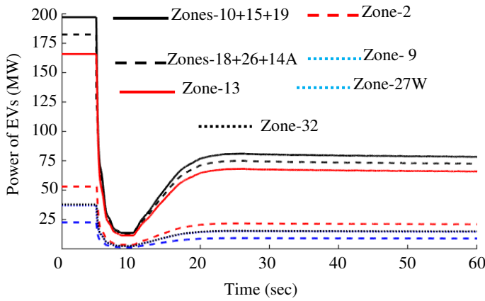
Fig.10 Power EVs at different zones
