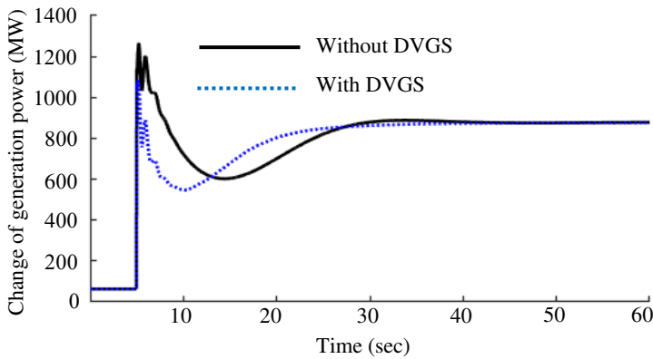
Fig.12 Change of power output ( \Delta P ) of aggregated generators
