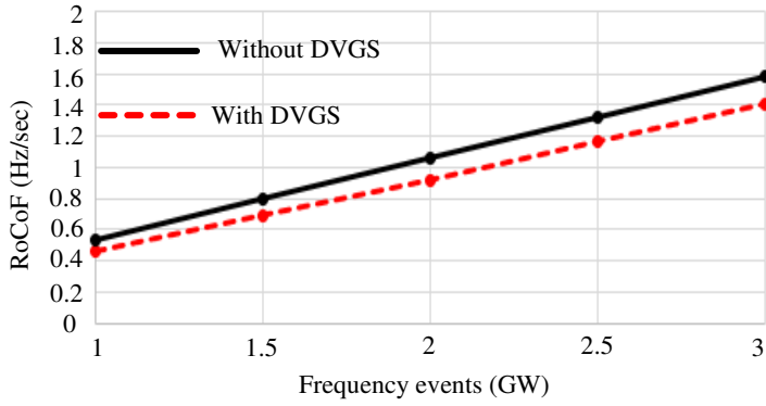
Fig. 16 Rate of change of frequency without DVGS model at 0.2sec following the event
