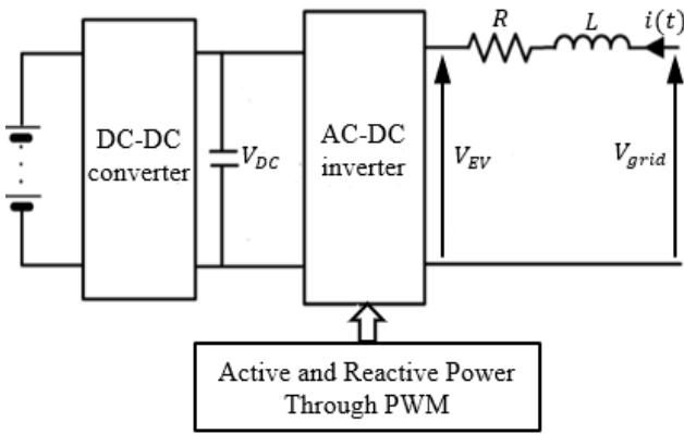
Fig. 1 The generic EV charging system
