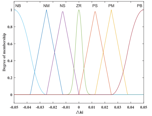
(b) Fuzzy sets of output variable \Delta k_i .
