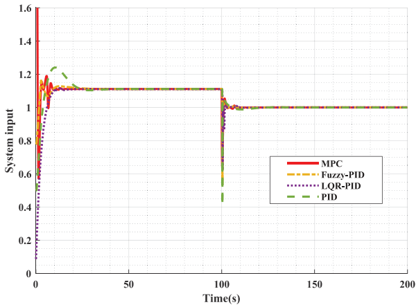
(b) The system input (the control variable u ).
