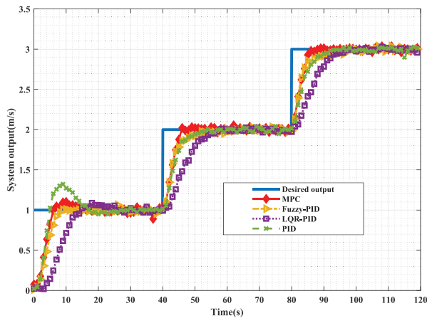
(a) The system output (the flow rate)
