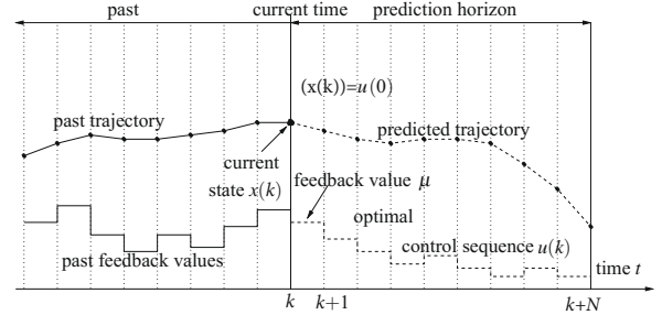
Figure 4: The working mechanism of the MPC at time t_n .
