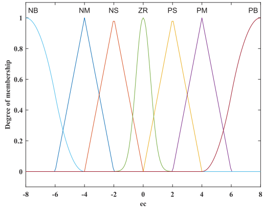
(b) Fuzzy sets of input variable ee .
