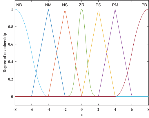
(a) Fuzzy sets of input variable e .
