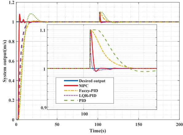
(a) The system output (the flow rate).
