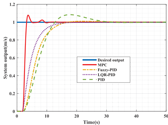
(a) The system output (the flow rate).
