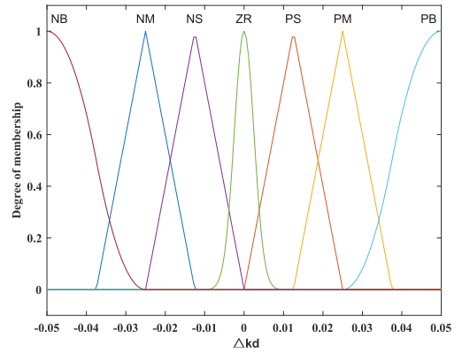
(c) Fuzzy sets of output variable \Delta k_d .
