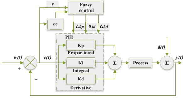
Figure 7: Illustration of the Fuzzy-PID Controller.
