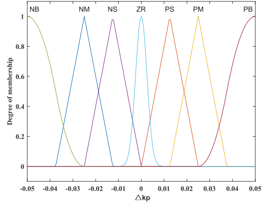
(a) Fuzzy sets of output variable \Delta k_p .
