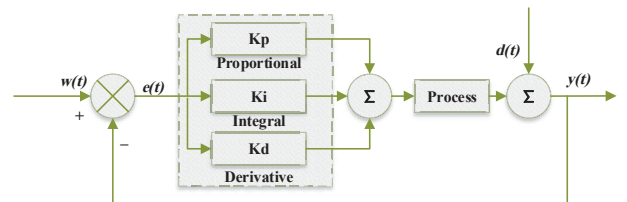
Figure 6: Illustration of the conventional PID controller.
