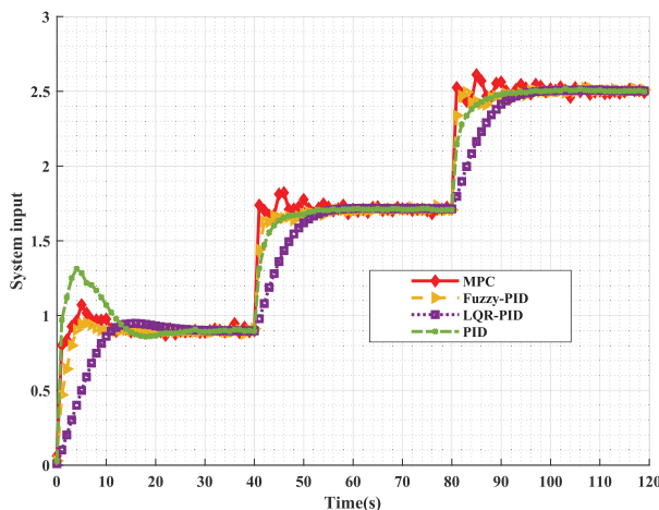
(b) The system input (the control variable u )
