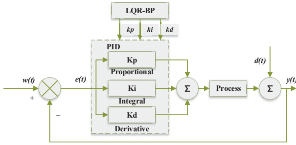
Figure 10: Illustration of the LQR-PID controller.
