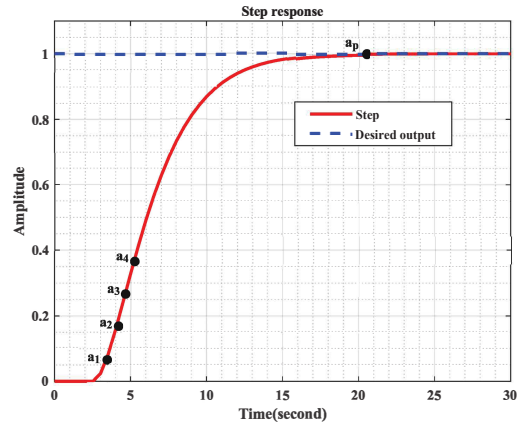
Figure 5: The step response curve of the slurry pipeline transportation system.
