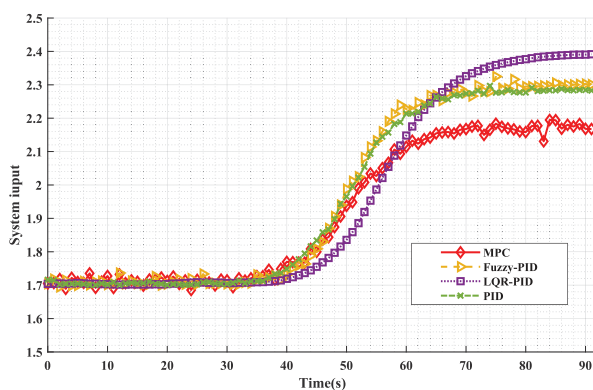
(b) The system input (the control variable u )
