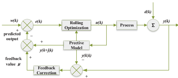
Figure 3: The control framework of the MPC approach.
