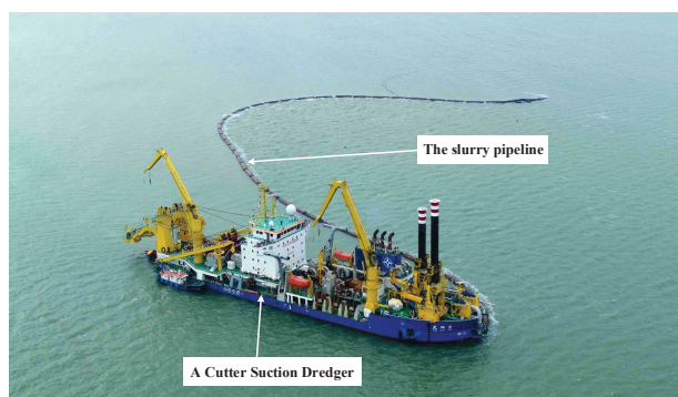
Figure 1: The cutter suction dredger with the slurry pipeline transportation system.
