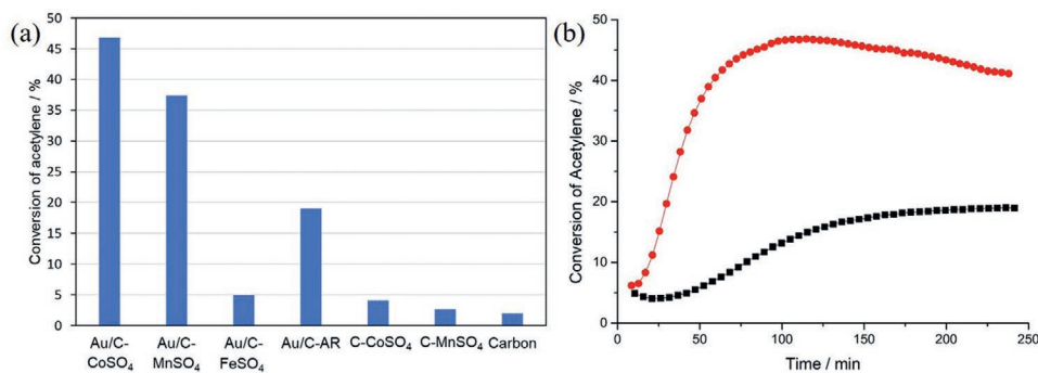
Figure 1. a) Comparison of acetylene conversions for Au/C- \text{CoSO}_4 , Au/C- \text{MnSO}_4 , and Au/C- \text{FeSO}_4 catalysts and their respective treated carbons. b) Au/C- \text{CoSO}_4 time-on-line data—Au/C- \text{CoSO}_4 (●), Au/C-AR (■).
