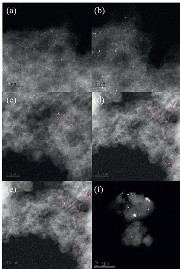
Figure 6. HAADF-STEM images of pre-wash 0.76 M H 2 SO 4 a,b) fresh, c,d) used at 160 °C, and e) used at 200 °C. f) FEG-SEM image of pre-wash 0.76 M H 2 SO 4 used at 200 °C.
