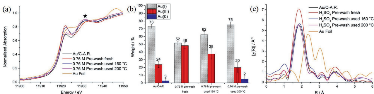
Figure 5. a) Au L 3 -edge XANES of Au/C-AR, pre-wash 0.76 M H 2 SO 4 fresh, used at 160 °C, and used at 200 °C and Au foil reference. ★ symbol shows position of second prominent scattering feature >11 930 eV. b) Linear combination fitting of the Au L 3 -edge XANES for the fresh aqua regia catalyst, fresh and used at 160 °C, and 200 °C 0.76 M H 2 SO 4 pre-wash catalysts. c) Fourier transform of the k 3 -weighted \chi EXAFS data of Au/C-AR, pre-wash 0.76 M H 2 SO 4 fresh, used at 160 °C, and used at 200 °C and Au foil reference.
