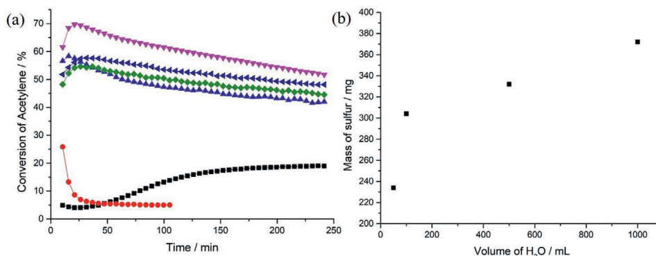
Figure 7. a) Acid pre-wash catalysts with varying volumes of H 2 O wash time-on-line data—Au/C-AR (■), 0 mL wash (●), 50 mL wash (▲), 100 mL wash (▼), 500 mL wash (◆), and 1000 mL wash (◀). b) Mass of sulfur removed from 0.76 M H 2 SO 4 pre-wash catalyst as determined by MP-AES versus volume of water used to wash catalyst.
