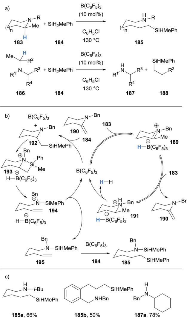
Scheme 34 Borane-mediated hydride abstraction utilised in a B(C_6F_5)_3 -catalysed cine -silylative ring opening and tertiary amines deconstruction processes.
