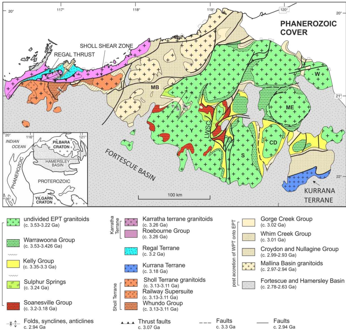
Fig. 1: Simplified geological map of the northern Pilbara Craton, showing greenstones and granitoids of the East Pilbara Terrane, Kurrana Terrane, Karraatha Terrane, Regal Terrane, Sholl Terrane and the late volcano-sedimentary Mallina Basin and De Grey Supergroup (MB=Mallina Basin; MCB=Mosquito Creek basin) and Fortescue Basin. Abbreviations for different granitoids that were sampled in this study: CD=Corunna Downs; ME=Mount Edgar; S=Shaw; W=Warrawagine; Y=Yule. Modified after Van Kranendonk et al., (2007a), (2010).
