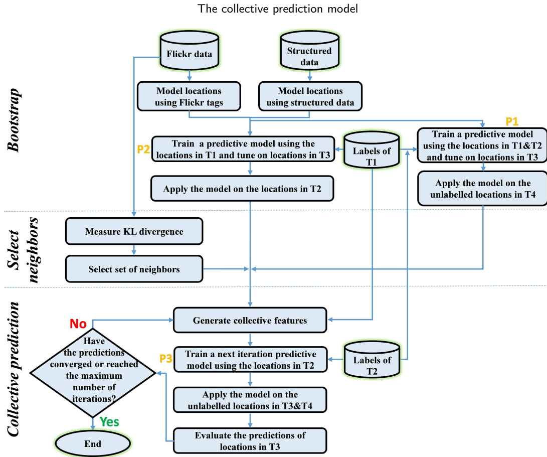
Figure 2: The collective prediction model.
