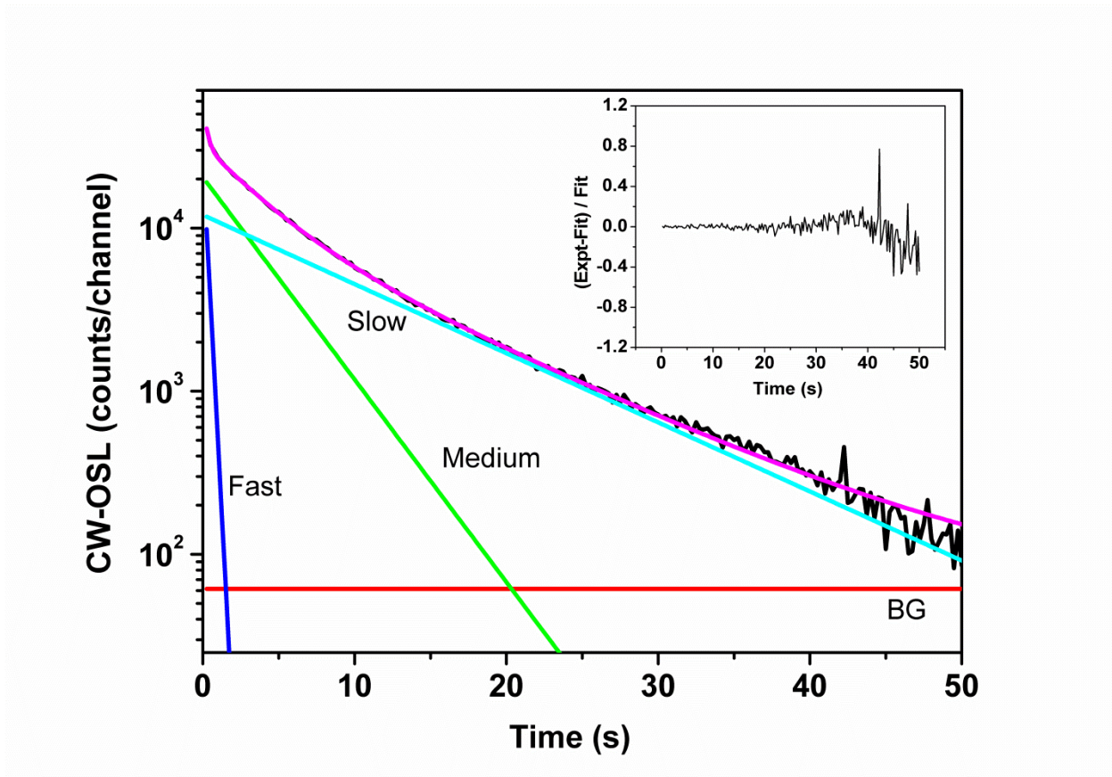
Fig.7. The experimentally obtained CW-OSL curve (in black) and theoretically fitted exponential decay curve (in pink) for CaSO 4 :Eu@900 phosphor (exposed to 1 Gy dose from Sr 90 /Y 90 beta source). The three components are shown in blue, green and light blue. The variation of (Expt.-Fit)/Fit with time is shown in the inset.
