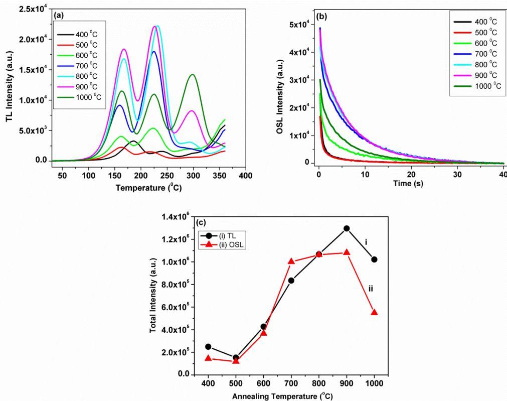
Fig. 3. (a) TL glow curves and (b) CW-OSL curves of \text{CaSO}_4:\text{Eu} nanophosphor annealed for 2 h at different temperatures ( 400\text{ }^\circ\text{C} to 1000\text{ }^\circ\text{C} ) for an absorbed dose of 1 Gy from \text{Sr}^{90}/\text{Y}^{90} beta source. (c) Effect of annealing temperature on the (i) TL response (ii) CW-OSL response of the \text{CaSO}_4:\text{Eu} phosphor.
