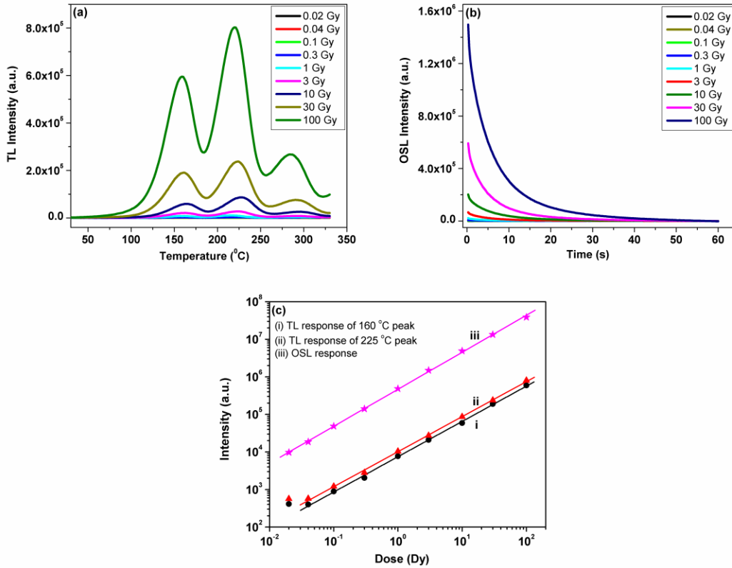
Fig. 5 (a) TL glow curves and (b) CW-OSL curves of CaSO 4 :Eu@900 phosphor. (c) Dose vs. TL and OSL response of CaSO 4 :Eu@900 phosphor (i) TL response of 160 °C peak (slope of fitted line = 0.94) (ii) TL response of 225 °C peak (slope of fitted line = 0.94) (iii) OSL response (total OSL intensity vs. dose) (slope of fitted line = 0.985). CaSO 4 :Eu@900 phosphor exposed to Sr 90 /Y 90 beta source at the different doses from 0.02 Gy to 100 Gy. The correlation coefficient (R 2 ) of the linear fits for all curves is found to be 0.999.
