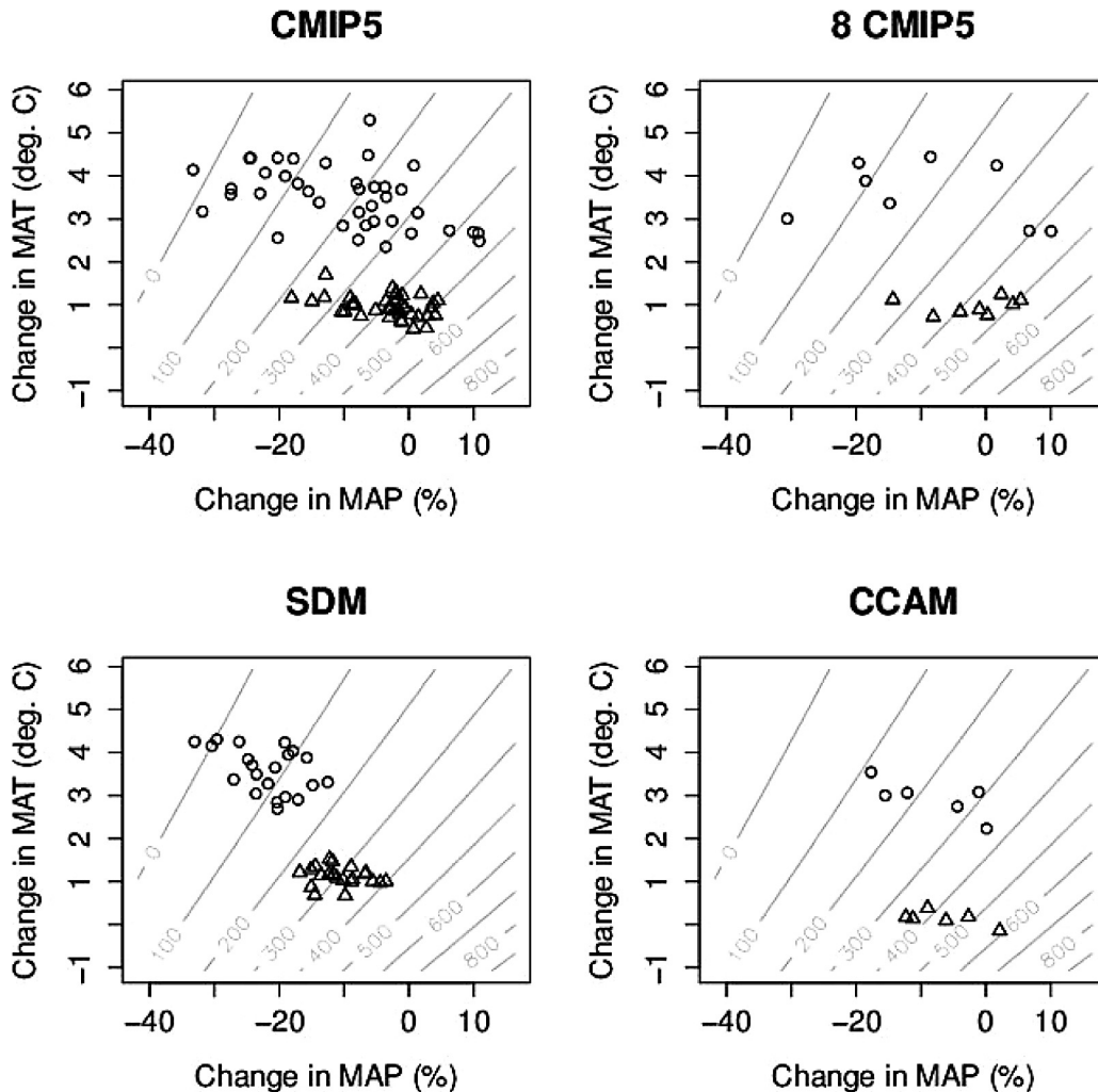
Fig. 8. For the catchment area (Fig. 4a): mean surface temperature (MAT, °C), mean annual precipitation (MAP, %) for 2080–2099 (circles) and 2020–2039 (triangles) relative to 1986–2005 for CMIP5 GCMs, 8 selected GCMs, SDM (21 models) and CCAM (6 models). Corresponding system yield (GL/yr) is indicated by grey lines.
