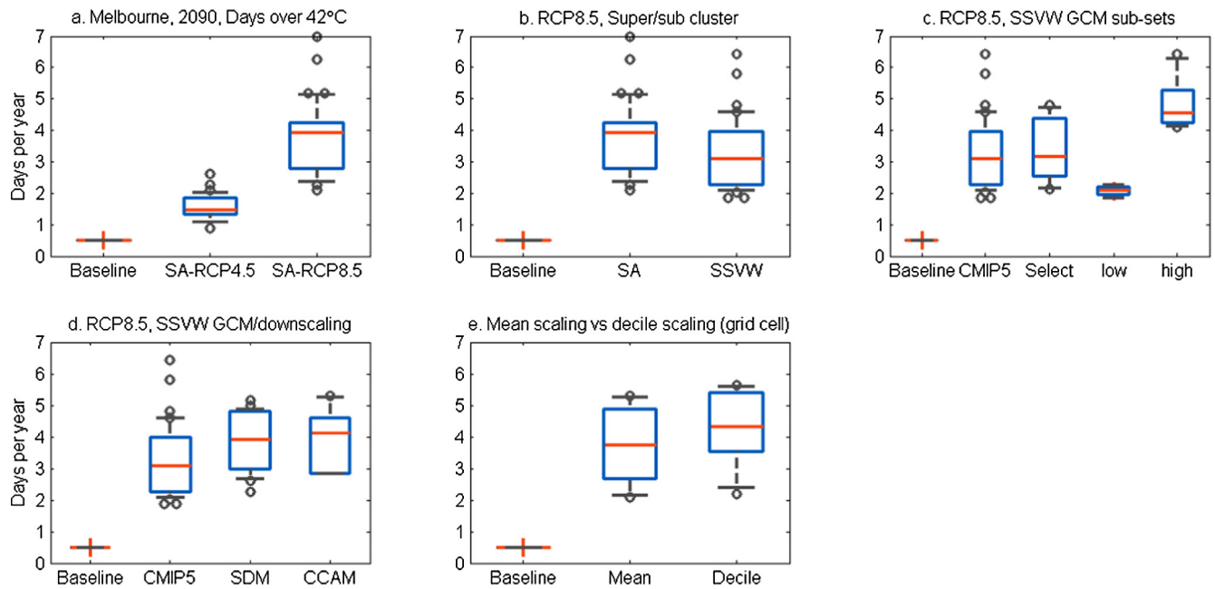
Fig. 2. Incidence of days over 42 °C in Melbourne in 1985–2005 (baseline) and 2090 under RCP8.5 calculated using different methods of scaling of the Melbourne ACORN-SAT station data series: (a) mean scaling factor from CMIP5 for Southern Australia (SA) super-cluster under RCP4.5 compared to RCP8.5, (b) mean scaling factor for CMIP5 for SA super-cluster and the Southern Slopes Victoria West (SSVW) sub-cluster, (c) mean scaling factor for SSVW in CMIP5, the 8 selected CMIP5 models, the 8 models showing the coolest temperature projection (low) and the eight with the hottest (high), (d) mean scaling factors for SSVW for CMIP5, BOM-SDM and CCAM downscaling, (e) mean and quantile scaling for the nearest GCM grid cell for the eight selected CMIP5 models (under RCP8.5).
