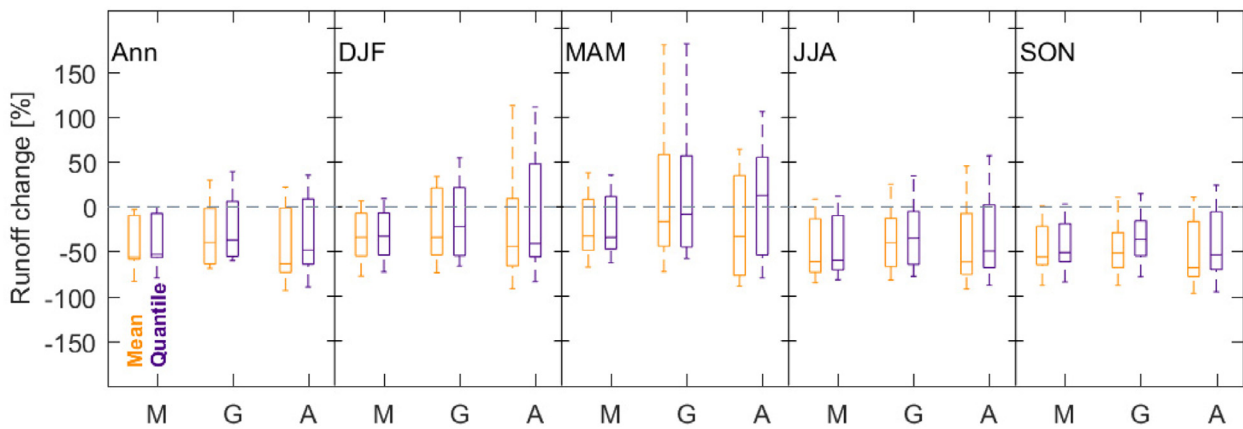
Fig. 6. Annual and seasonal runoff change (%) for 2080–2099 relative to 1986–2005 following RCP8.5 for three catchments (M = Murray, G = Genoa and A = Avoca, see Fig. 2). Orange bars indicate hydrological model inputs of mean scaled application-ready data for rainfall and APET, and purple bars indicate inputs of quantile scaled rainfall and mean scaled APET.
