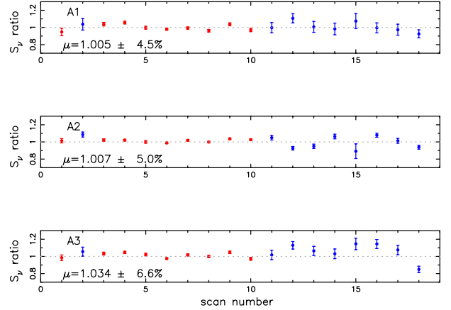
Fig. 17. Comparison of measured and reference flux densities of the primary calibrators Uranus (red) and Neptune (blue). Their ratios are shown for the three arrays A1 (260 GHz-H), A2 (150 GHz), and A3 (260 GHz-V). The mean ratio \mu and relative scatter are provided for each array. The reference flux densities are from Moreno (2010), Bendo et al. (2013). The scan numbers are time-ordered: 1 to 10 refer the period 23–28 February, 2017 (fair weather) and 11 to 18 to the period 19–25 April, 2017 (mediocre weather).
