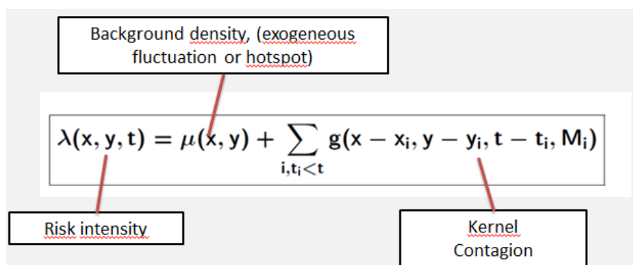
Figure 1: Predicting occurrence
