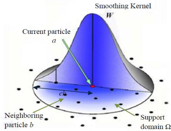
Fig. 1. Particle approximations using neighbouring particles within the support domain of the smoothing kernel W for particle a [3]
